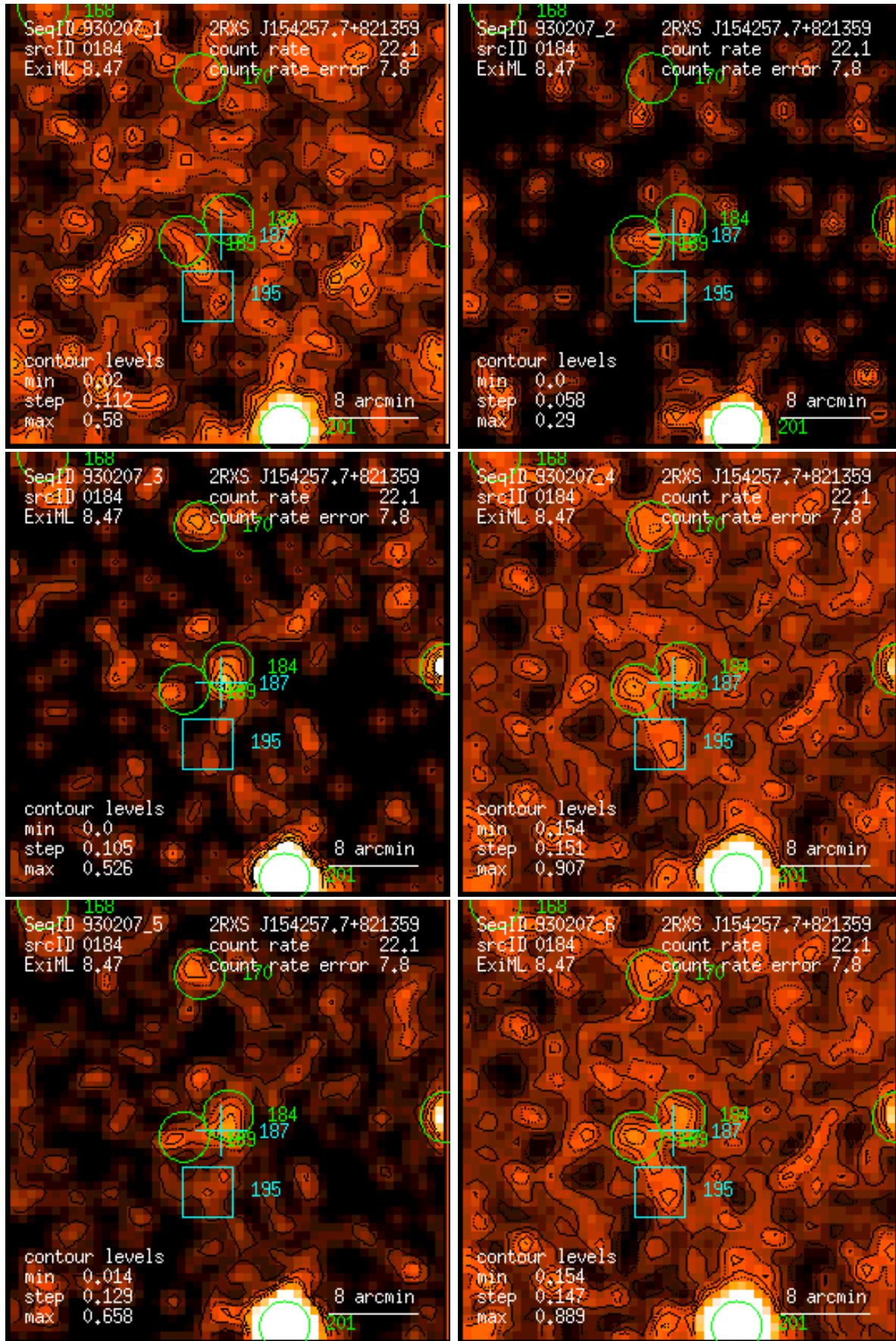
Figure 184: RASS 930207: detection 0184: band rate images, Gaussian filter: (1) PSPC channels 11 – 41, (2) 52 – 90, (3) 91 – 201, (4) 11 – 235, (5) 52 – 201, (6) 11 – 201. Broad band rates in counts/ks. Band rate contour levels in counts/ks/arcmin 2 .
