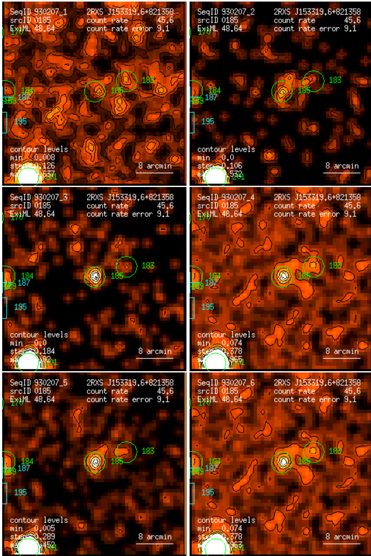
Figure 185: RASS 930207: detection 0185: band rate images, Gaussian filter: (1) PSPC channels 11 – 41, (2) 52 – 90, (3) 91 – 201, (4) 11 – 235, (5) 52 – 201, (6) 11 – 201. Broad band rates in counts/ks. Band rate contour levels in counts/ks/arcmin 2 .
