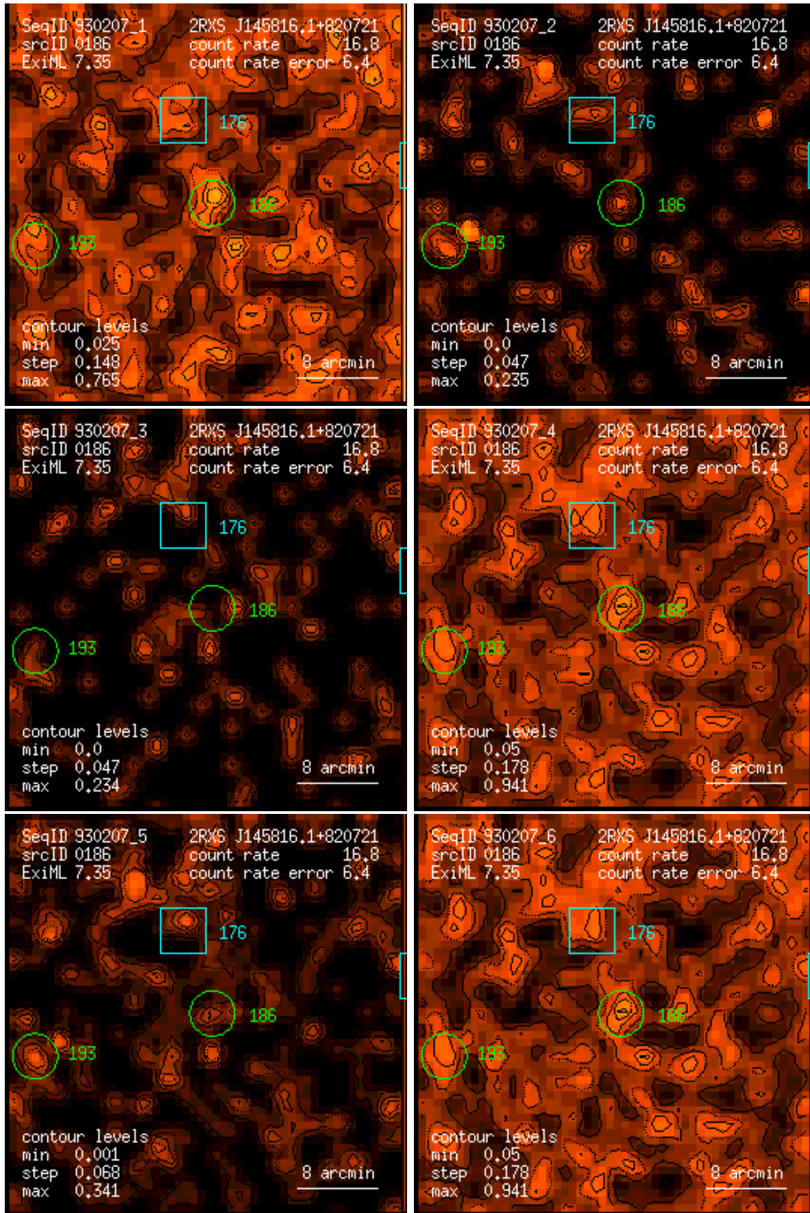
Figure 186: RASS 930207: detection 0186: band rate images, Gaussian filter: (1) PSPC channels 11 – 41, (2) 52 – 90, (3) 91 – 201, (4) 11 – 235, (5) 52 – 201, (6) 11 – 201. Broad band rates in counts/ks. Band rate contour levels in counts/ks/arcmin 2 .
