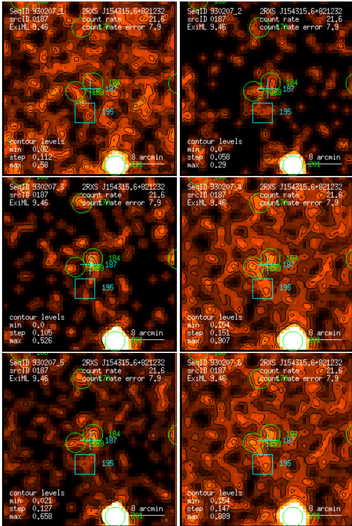
Figure 187: RASS 930207: detection 0187: band rate images, Gaussian filter: (1) PSPC channels 11 – 41, (2) 52 – 90, (3) 91 – 201, (4) 11 – 235, (5) 52 – 201, (6) 11 – 201. Broad band rates in counts/ks. Band rate contour levels in counts/ks/arcmin 2 .
