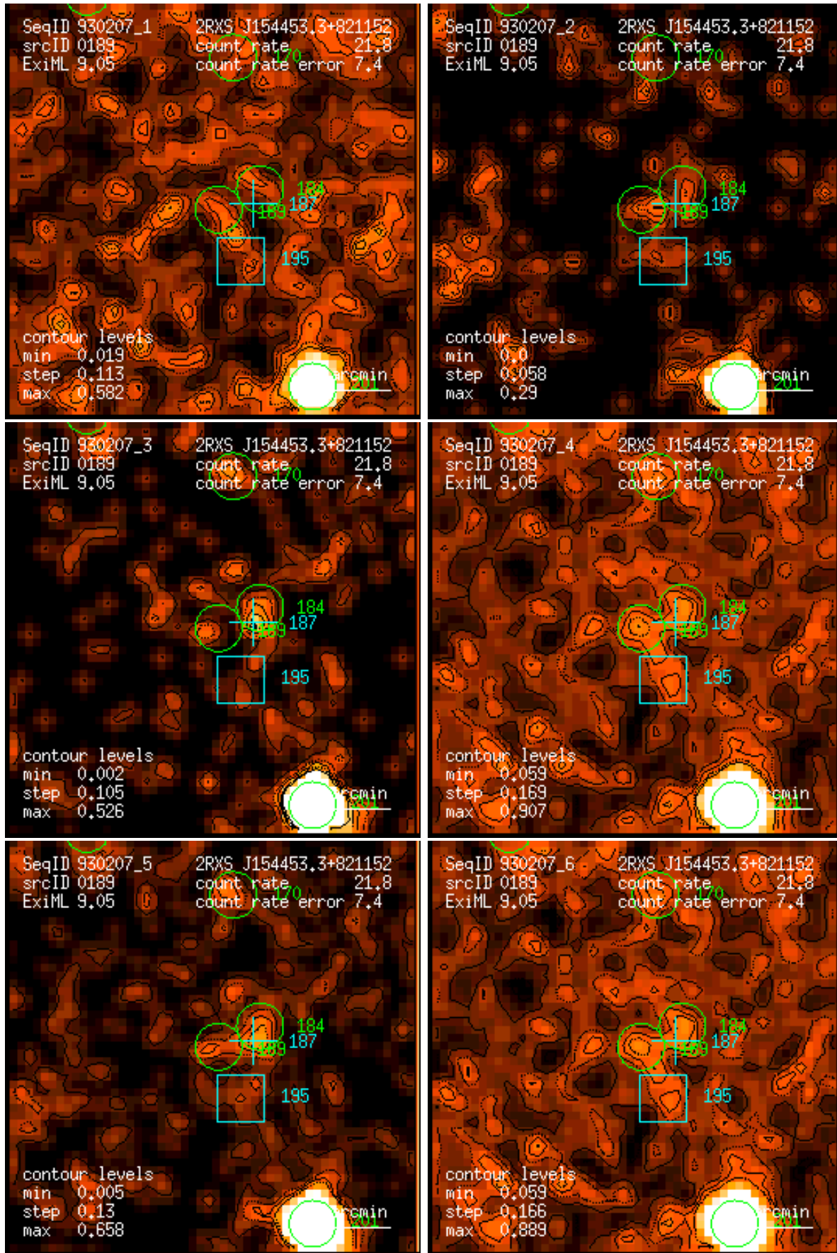
Figure 189: RASS 930207: detection 0189: band rate images, Gaussian filter: (1) PSPC channels 11 – 41, (2) 52 – 90, (3) 91 – 201, (4) 11 – 235, (5) 52 – 201, (6) 11 – 201. Broad band rates in counts/ks. Band rate contour levels in counts/ks/arcmin 2 .
