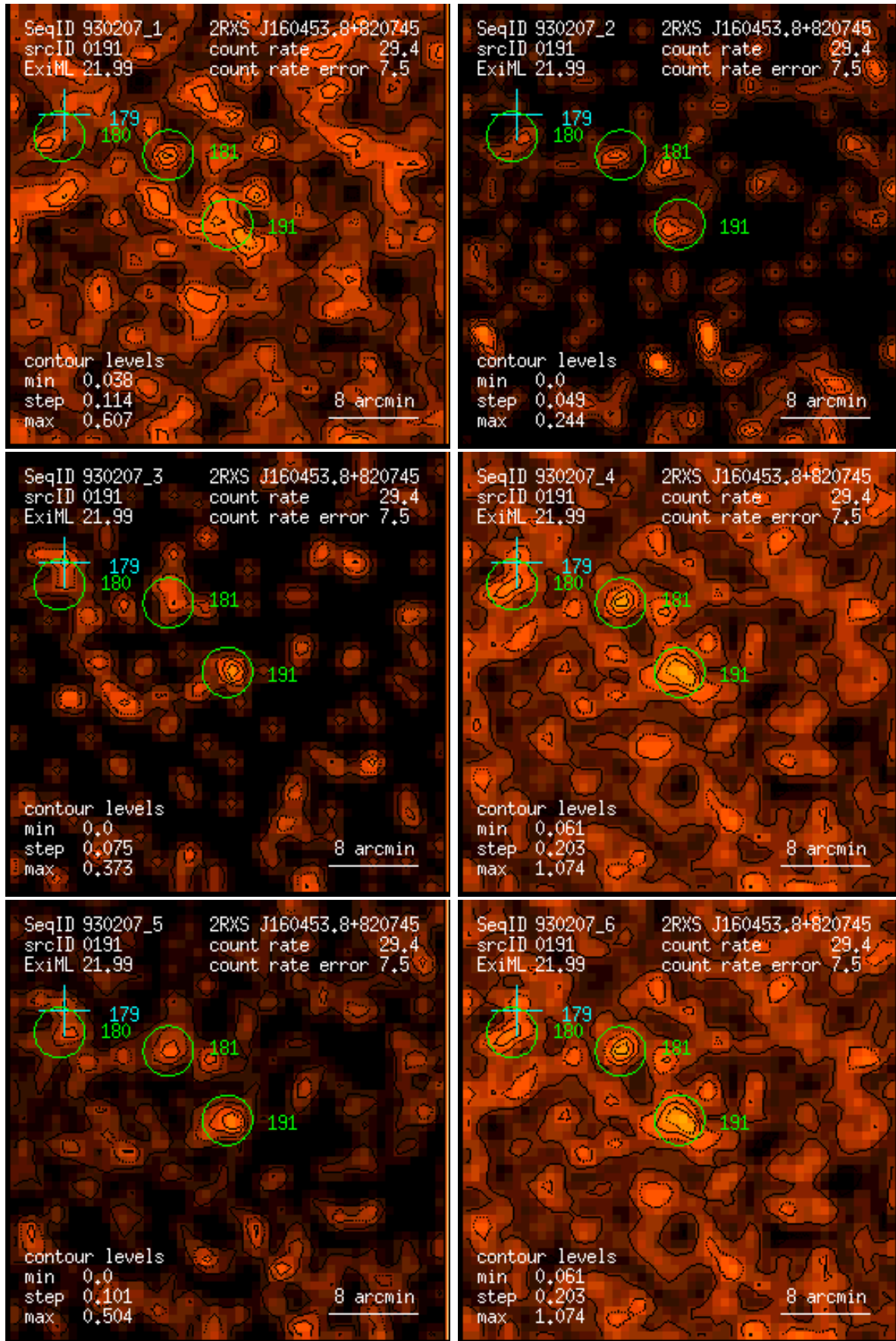
Figure 191: RASS 930207: detection 0191: band rate images, Gaussian filter: (1) PSPC channels 11 – 41, (2) 52 – 90, (3) 91 – 201, (4) 11 – 235, (5) 52 – 201, (6) 11 – 201. Broad band rates in counts/ks. Band rate contour levels in counts/ks/arcmin 2 .
