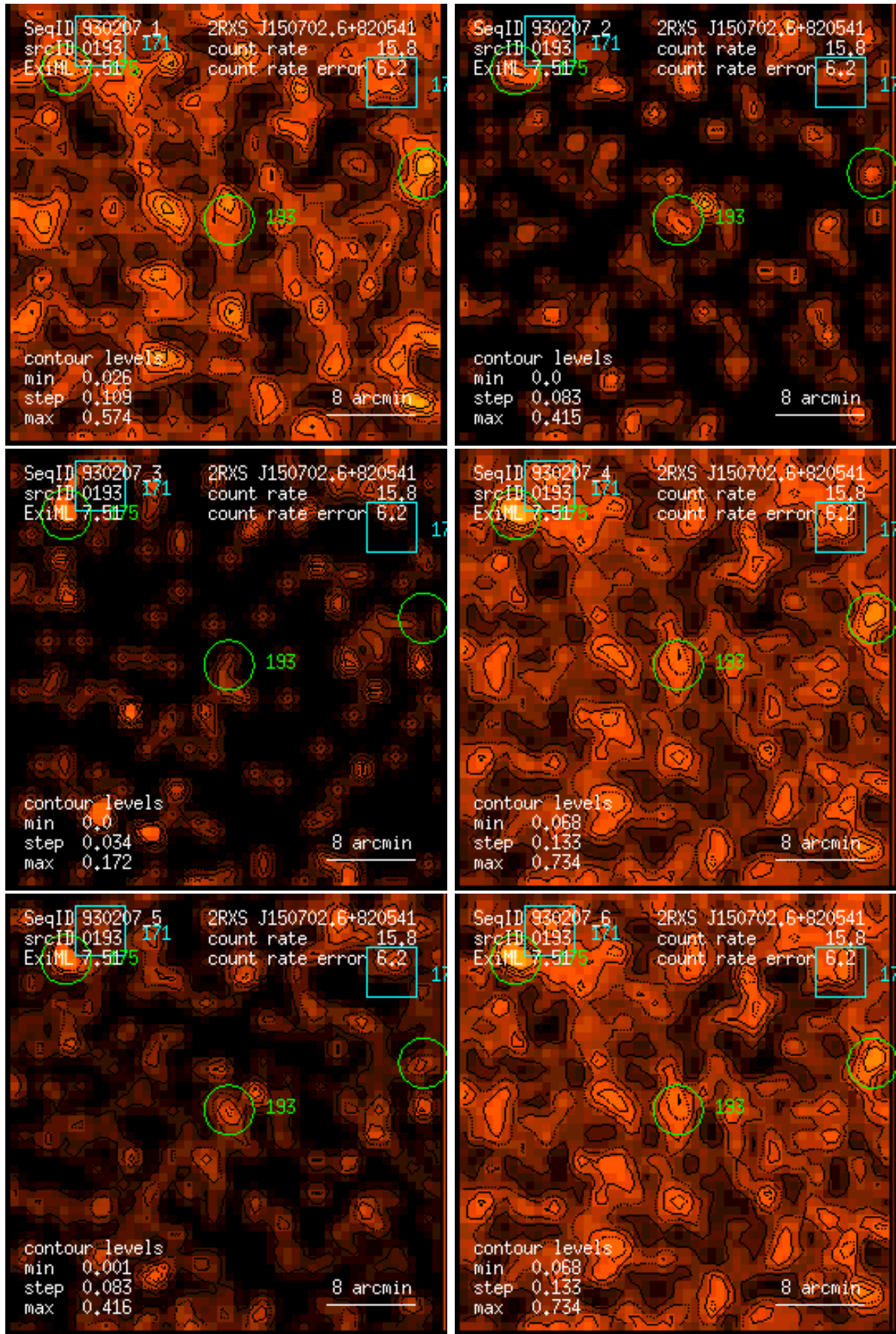
Figure 193: RASS 930207: detection 0193: band rate images, Gaussian filter: (1) PSPC channels 11 – 41, (2) 52 – 90, (3) 91 – 201, (4) 11 – 235, (5) 52 – 201, (6) 11 – 201. Broad band rates in counts/ks. Band rate contour levels in counts/ks/arcmin 2 .
