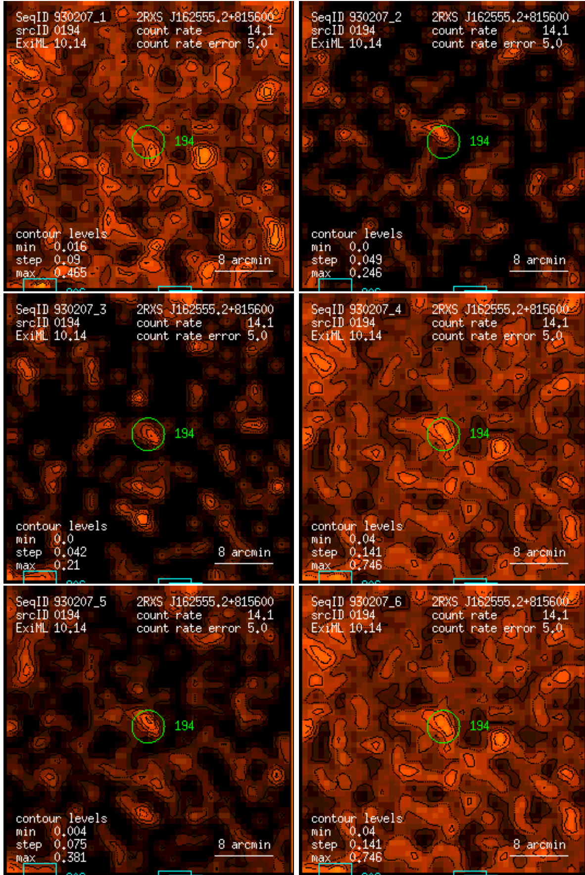
Figure 194: RASS 930207: detection 0194: band rate images, Gaussian filter: (1) PSPC channels 11 – 41, (2) 52 – 90, (3) 91 – 201, (4) 11 – 235, (5) 52 – 201, (6) 11 – 201. Broad band rates in counts/ks. Band rate contour levels in counts/ks/arcmin 2 .
