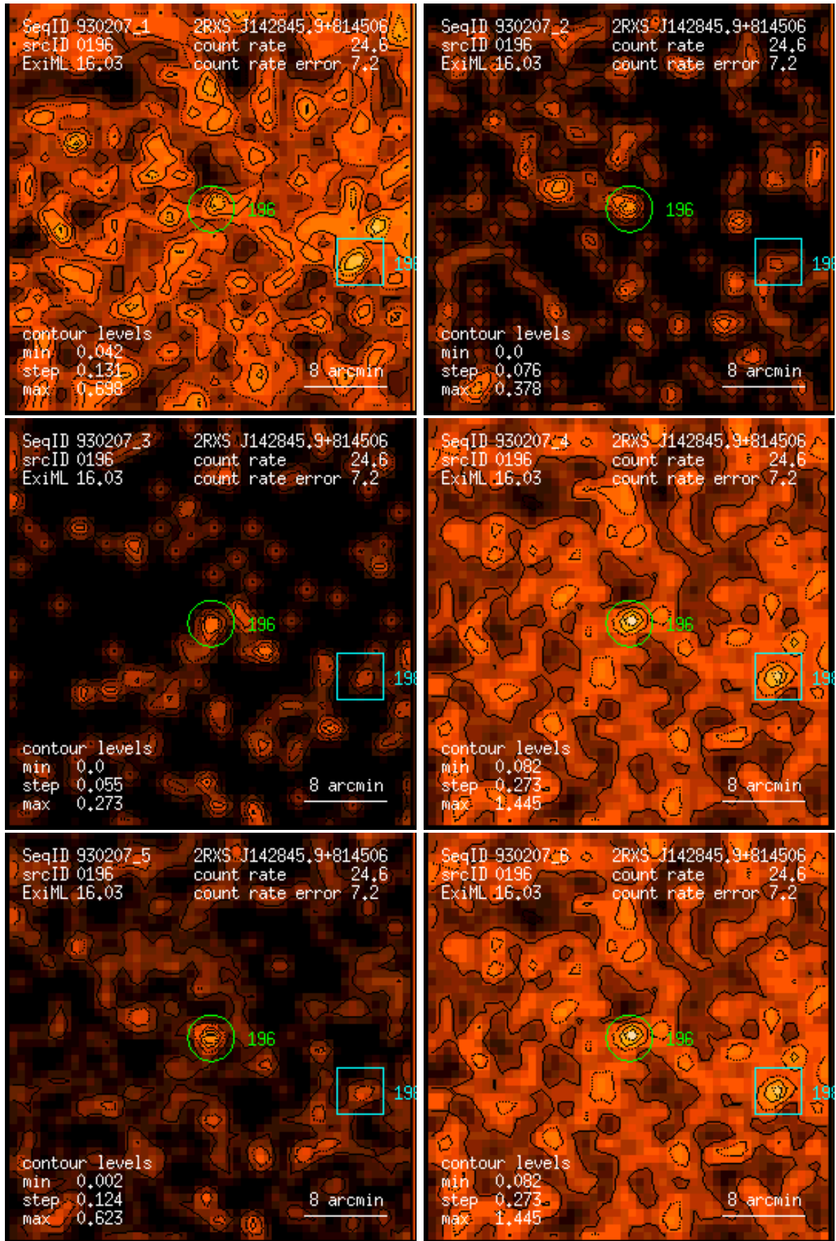
Figure 196: RASS 930207: detection 0196: band rate images, Gaussian filter: (1) PSPC channels 11 – 41, (2) 52 – 90, (3) 91 – 201, (4) 11 – 235, (5) 52 – 201, (6) 11 – 201. Broad band rates in counts/ks. Band rate contour levels in counts/ks/arcmin 2 .
