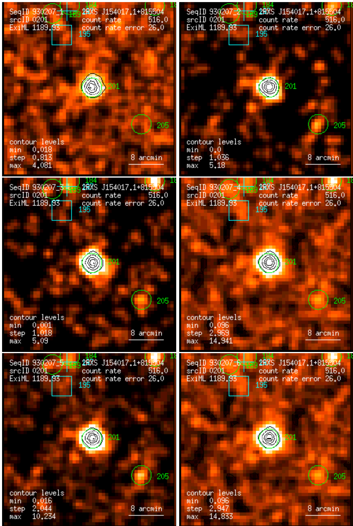
Figure 201: RASS 930207: detection 0201: band rate images, Gaussian filter: (1) PSPC channels 11 – 41, (2) 52 – 90, (3) 91 – 201, (4) 11 – 235, (5) 52 – 201, (6) 11 – 201. Broad band rates in counts/ks. Band rate contour levels in counts/ks/arcmin 2 .
