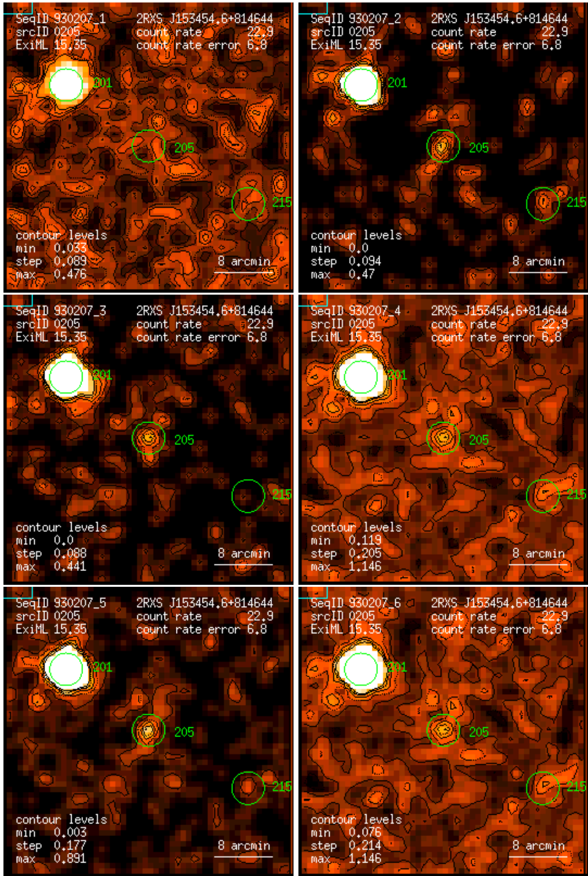
Figure 205: RASS 930207: detection 0205: band rate images, Gaussian filter: (1) PSPC channels 11 – 41, (2) 52 – 90, (3) 91 – 201, (4) 11 – 235, (5) 52 – 201, (6) 11 – 201. Broad band rates in counts/ks. Band rate contour levels in counts/ks/arcmin 2 .
