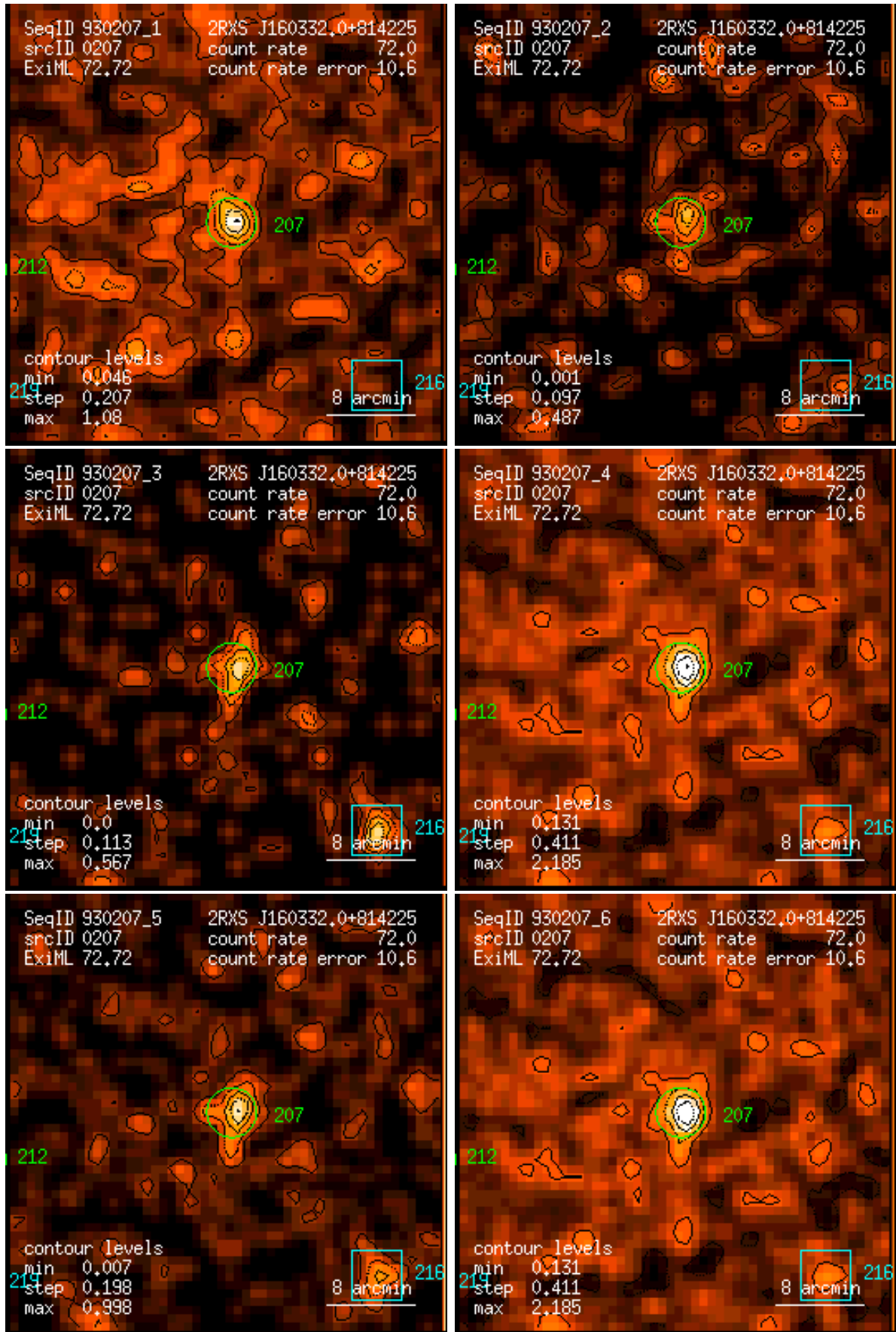
Figure 207: RASS 930207: detection 0207: band rate images, Gaussian filter: (1) PSPC channels 11 – 41, (2) 52 – 90, (3) 91 – 201, (4) 11 – 235, (5) 52 – 201, (6) 11 – 201. Broad band rates in counts/ks. Band rate contour levels in counts/ks/arcmin 2 .
