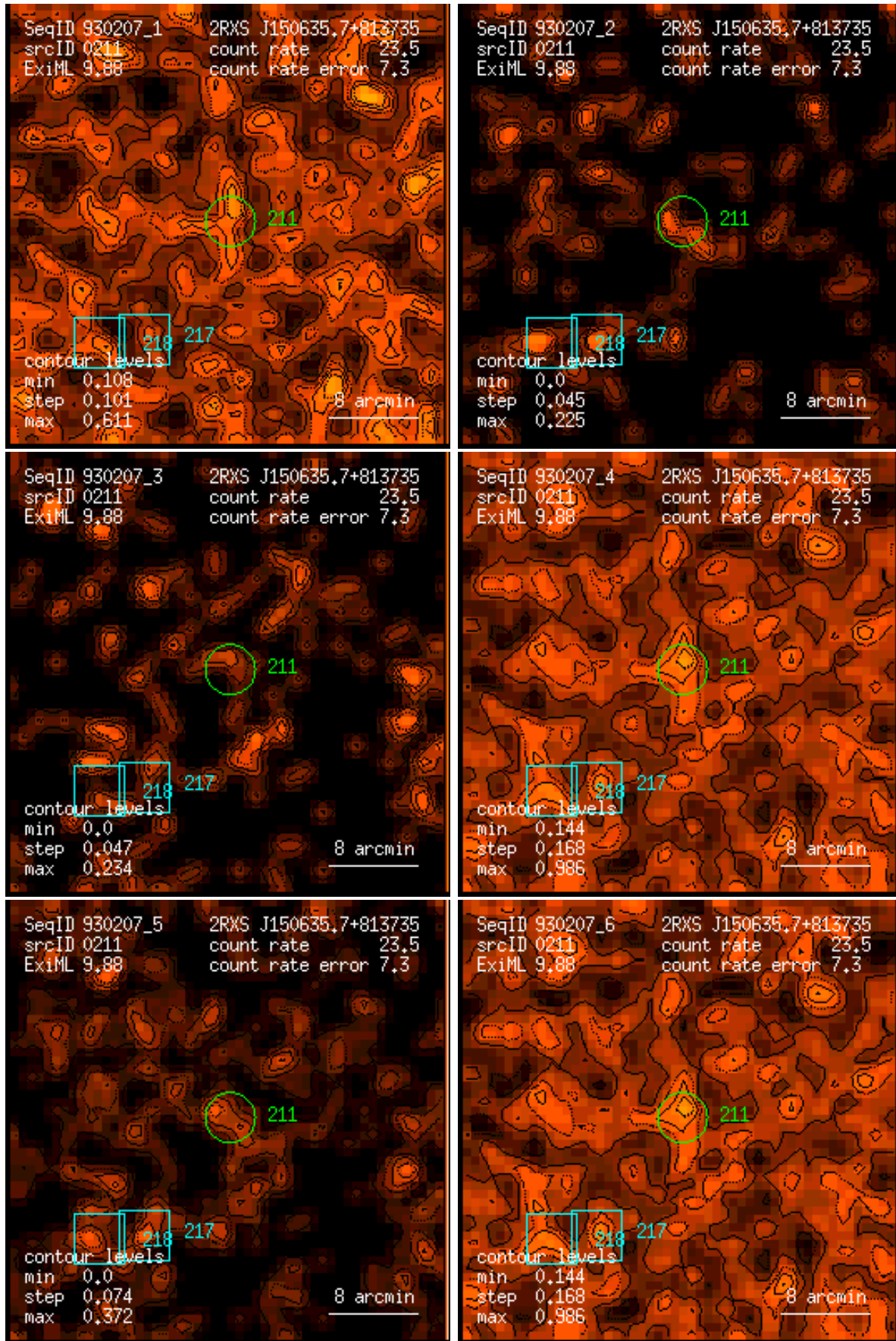
Figure 211: RASS 930207: detection 0211: band rate images, Gaussian filter: (1) PSPC channels 11 – 41, (2) 52 – 90, (3) 91 – 201, (4) 11 – 235, (5) 52 – 201, (6) 11 – 201. Broad band rates in counts/ks. Band rate contour levels in counts/ks/arcmin 2 .
