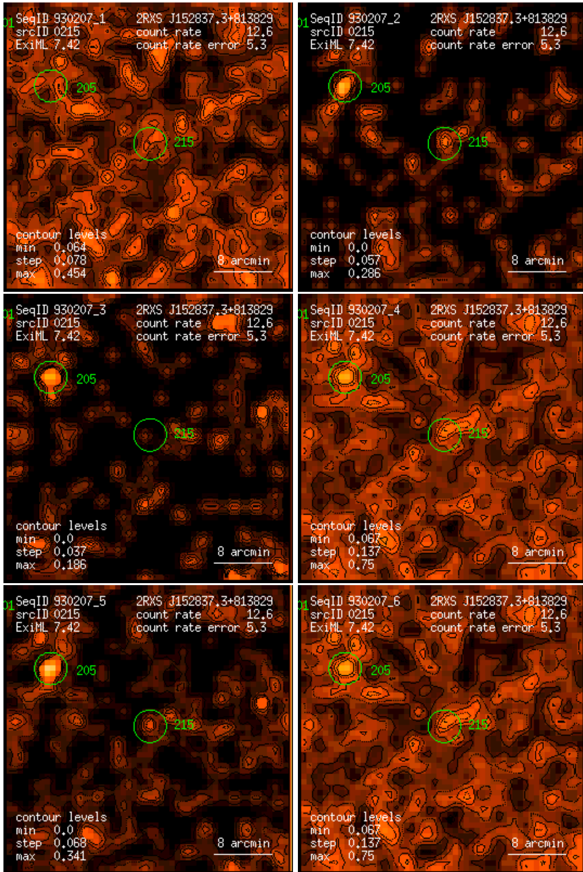
Figure 215: RASS 930207: detection 0215: band rate images, Gaussian filter: (1) PSPC channels 11 – 41, (2) 52 – 90, (3) 91 – 201, (4) 11 – 235, (5) 52 – 201, (6) 11 – 201. Broad band rates in counts/ks. Band rate contour levels in counts/ks/arcmin 2 .
