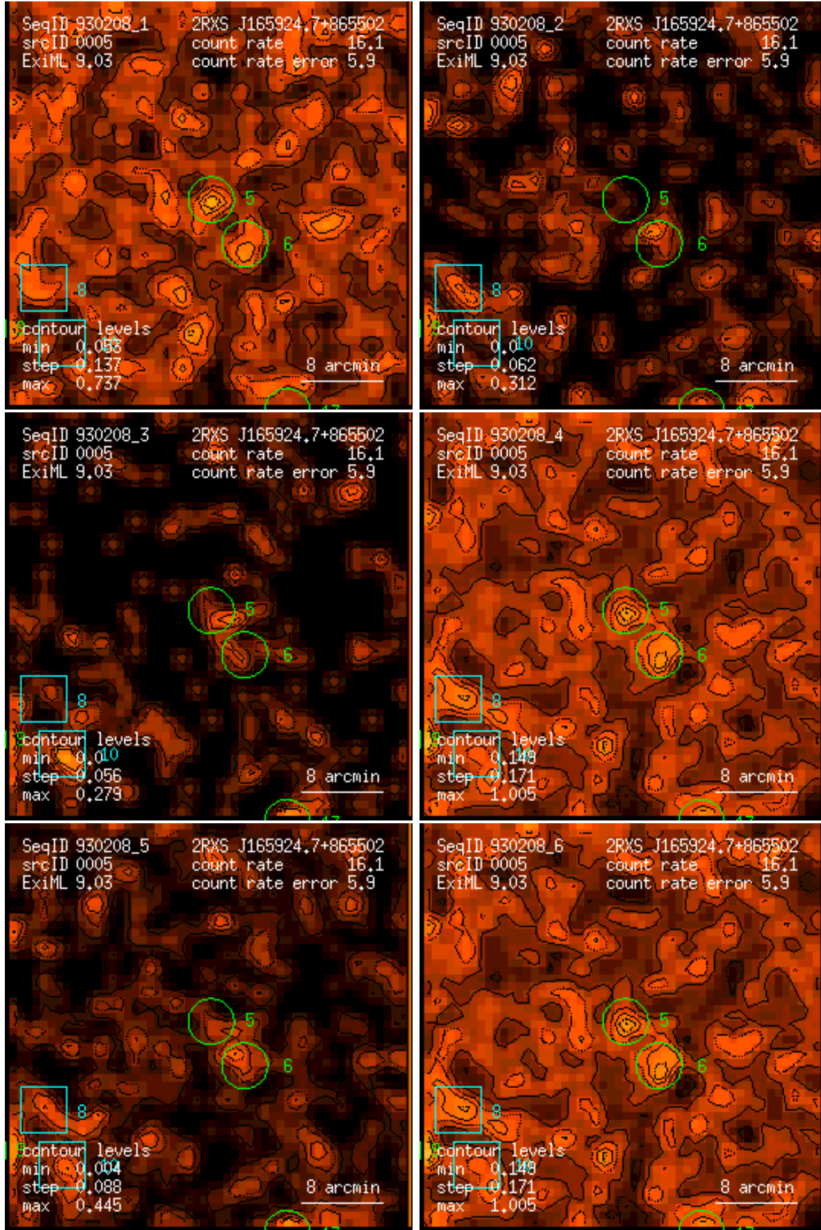
Figure 5: RASS 930208: detection 0005: band rate images, Gaussian filter: (1) PSPC channels 11 – 41, (2) 52 – 90, (3) 91 – 201, (4) 11 – 235, (5) 52 – 201, (6) 11 – 201. Broad band rates in counts/ks. Band rate contour levels in counts/ks/arcmin 2 .
