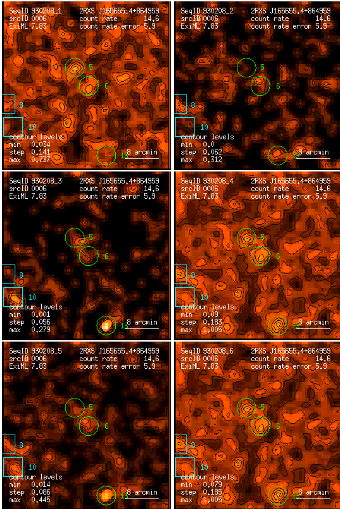
Figure 6: RASS 930208: detection 0006: band rate images, Gaussian filter: (1) PSPC channels 11 – 41, (2) 52 – 90, (3) 91 – 201, (4) 11 – 235, (5) 52 – 201, (6) 11 – 201. Broad band rates in counts/ks. Band rate contour levels in counts/ks/arcmin 2 .
