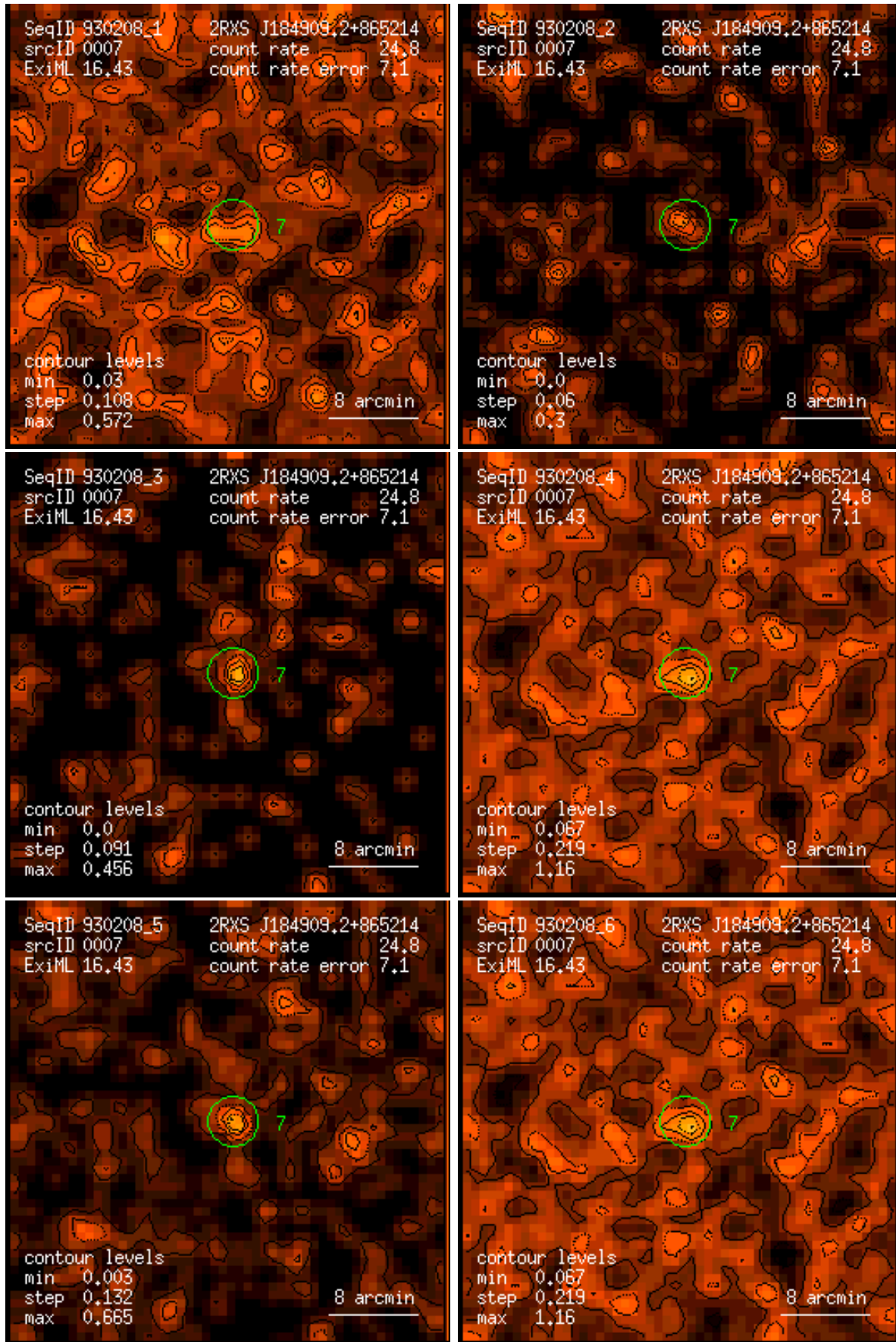
Figure 7: RASS 930208: detection 0007: band rate images, Gaussian filter: (1) PSPC channels 11 – 41, (2) 52 – 90, (3) 91 – 201, (4) 11 – 235, (5) 52 – 201, (6) 11 – 201. Broad band rates in counts/ks. Band rate contour levels in counts/ks/arcmin 2 .
