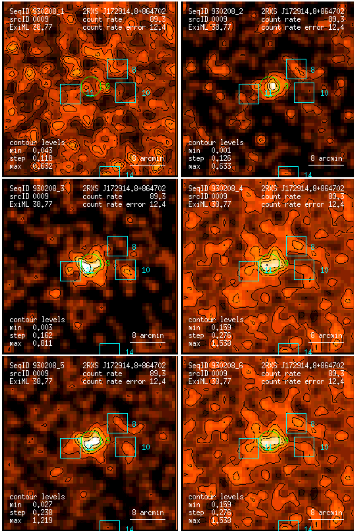
Figure 9: RASS 930208: detection 0009: band rate images, Gaussian filter: (1) PSPC channels 11 – 41, (2) 52 – 90, (3) 91 – 201, (4) 11 – 235, (5) 52 – 201, (6) 11 – 201. Broad band rates in counts/ks. Band rate contour levels in counts/ks/arcmin 2 .
