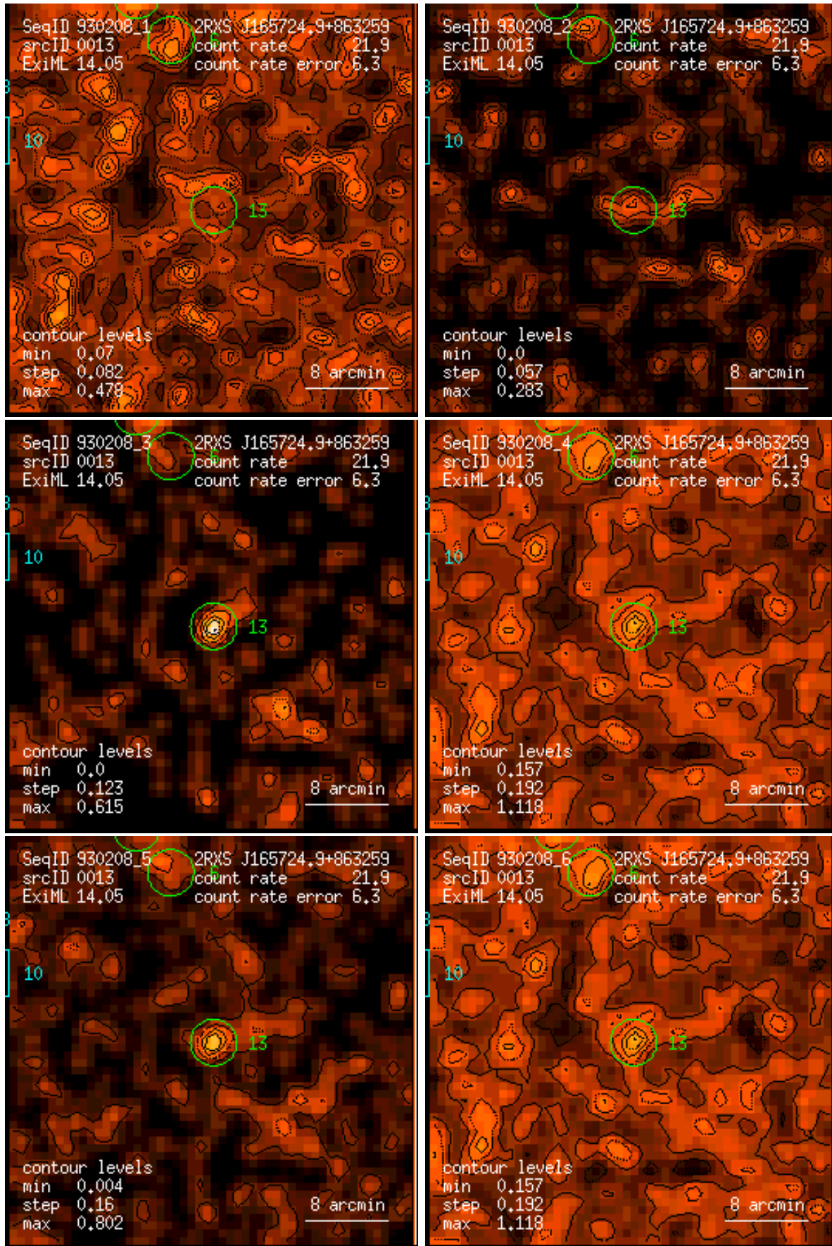
Figure 13: RASS 930208: detection 0013: band rate images, Gaussian filter: (1) PSPC channels 11 – 41, (2) 52 – 90, (3) 91 – 201, (4) 11 – 235, (5) 52 – 201, (6) 11 – 201. Broad band rates in counts/ks. Band rate contour levels in counts/ks/arcmin 2 .
