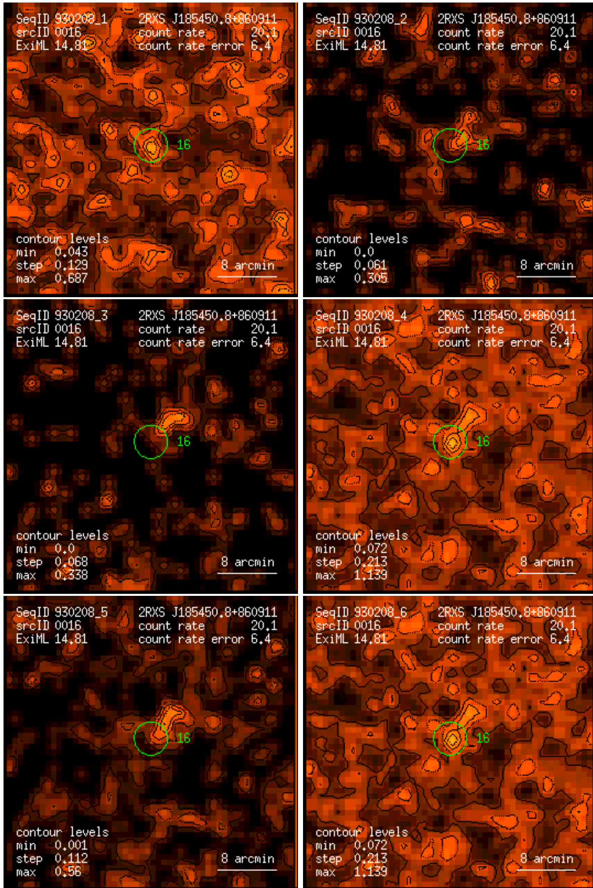
Figure 16: RASS 930208: detection 0016: band rate images, Gaussian filter: (1) PSPC channels 11 – 41, (2) 52 – 90, (3) 91 – 201, (4) 11 – 235, (5) 52 – 201, (6) 11 – 201. Broad band rates in counts/ks. Band rate contour levels in counts/ks/arcmin 2 .
