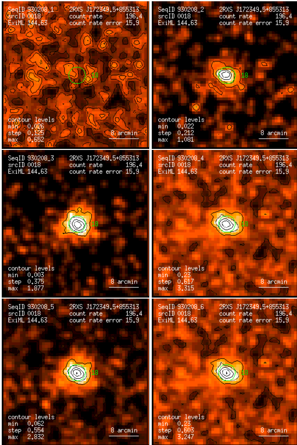
Figure 18: RASS 930208: detection 0018: band rate images, Gaussian filter: (1) PSPC channels 11 – 41, (2) 52 – 90, (3) 91 – 201, (4) 11 – 235, (5) 52 – 201, (6) 11 – 201. Broad band rates in counts/ks. Band rate contour levels in counts/ks/arcmin 2 .
