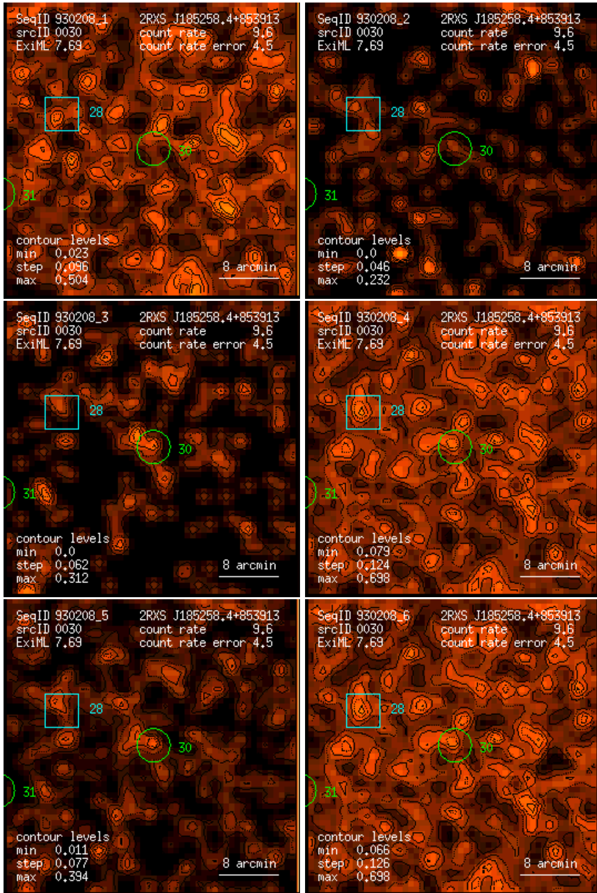
Figure 30: RASS 930208: detection 0030: band rate images, Gaussian filter: (1) PSPC channels 11 – 41, (2) 52 – 90, (3) 91 – 201, (4) 11 – 235, (5) 52 – 201, (6) 11 – 201. Broad band rates in counts/ks. Band rate contour levels in counts/ks/arcmin 2 .
