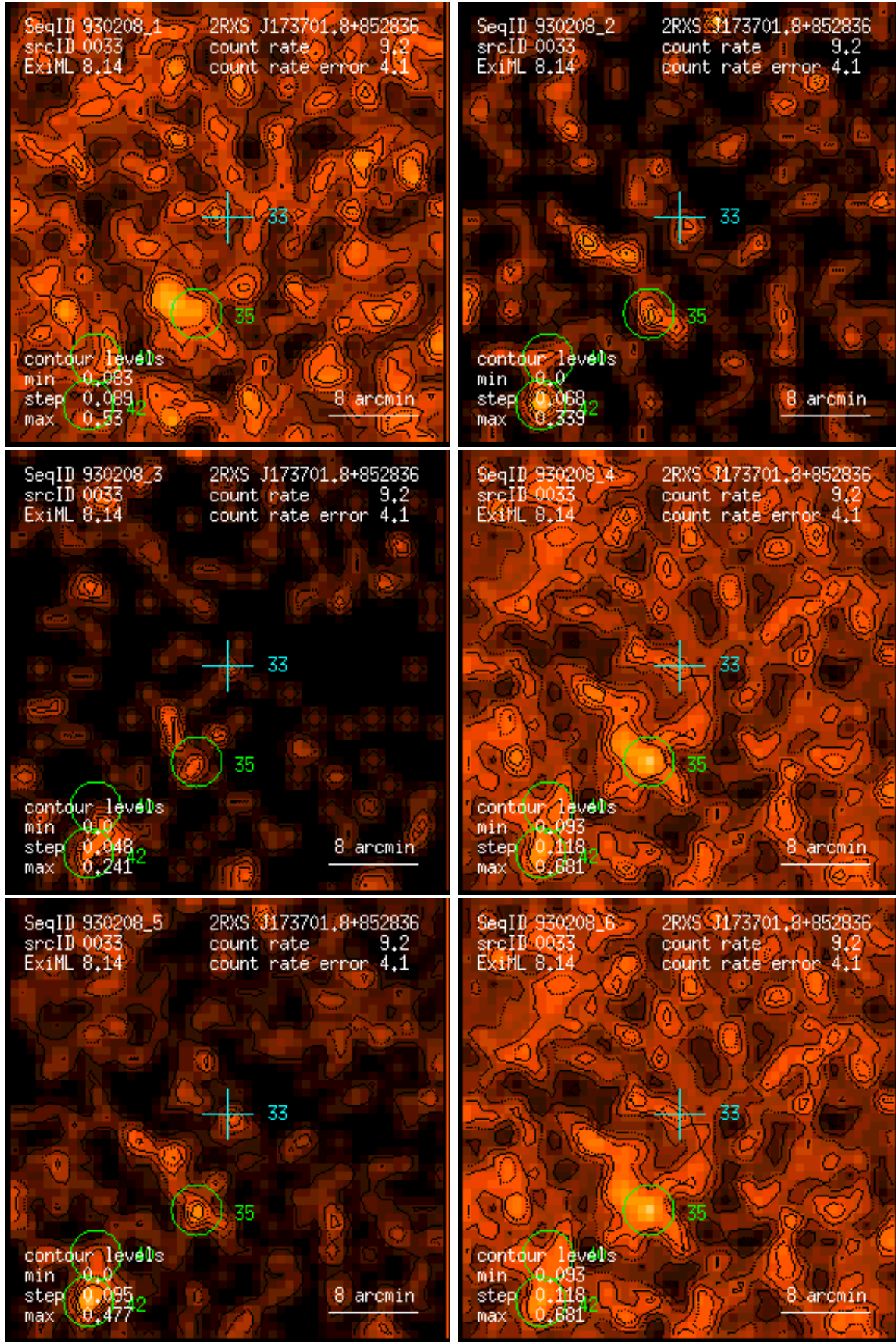
Figure 33: RASS 930208: detection 0033: band rate images, Gaussian filter: (1) PSPC channels 11 – 41, (2) 52 – 90, (3) 91 – 201, (4) 11 – 235, (5) 52 – 201, (6) 11 – 201. Broad band rates in counts/ks. Band rate contour levels in counts/ks/arcmin 2 .
