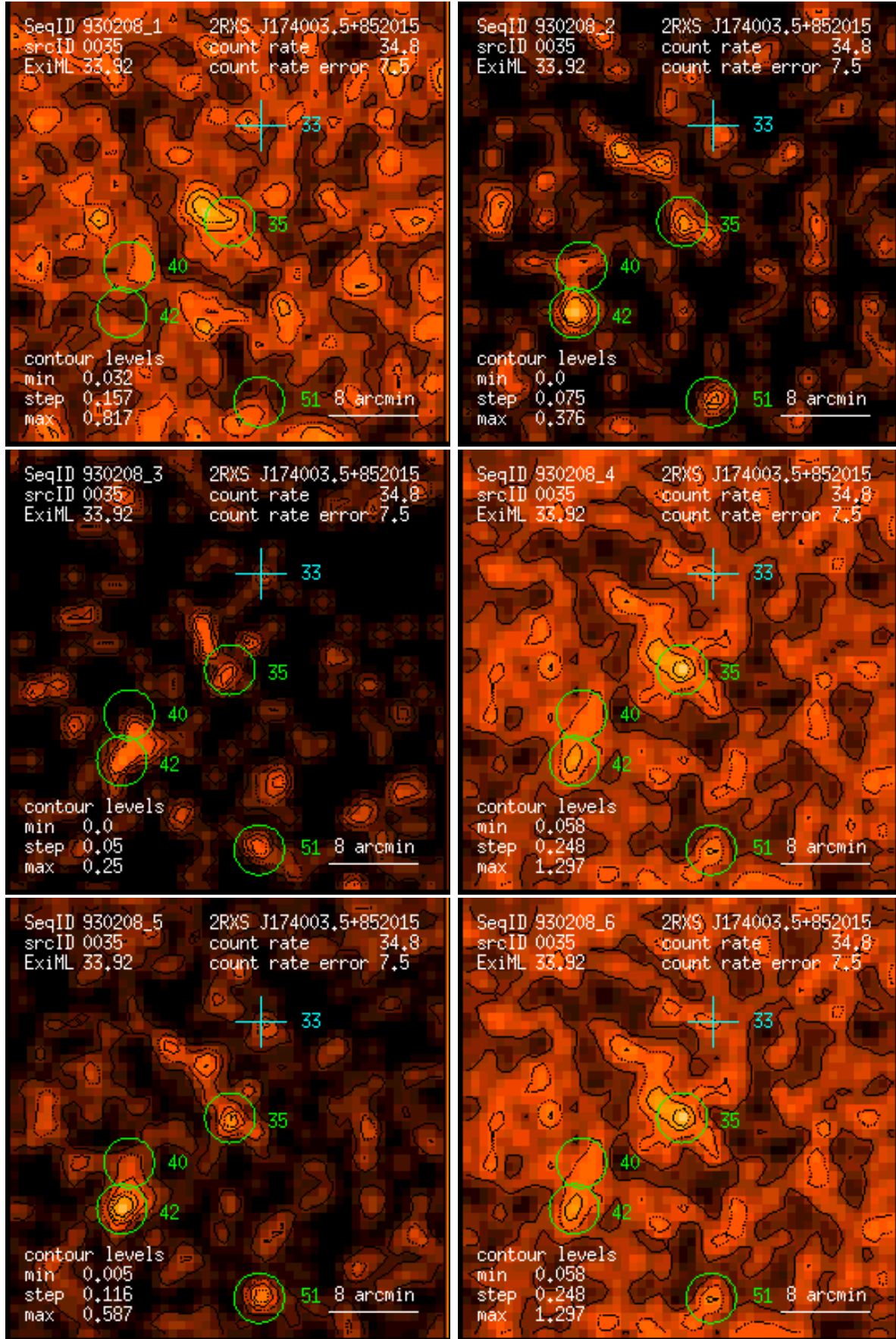
Figure 35: RASS 930208: detection 0035: band rate images, Gaussian filter: (1) PSPC channels 11 – 41, (2) 52 – 90, (3) 91 – 201, (4) 11 – 235, (5) 52 – 201, (6) 11 – 201. Broad band rates in counts/ks. Band rate contour levels in counts/ks/arcmin 2 .
