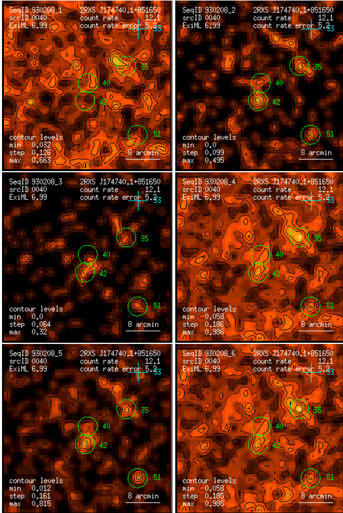
Figure 40: RASS 930208: detection 0040: band rate images, Gaussian filter: (1) PSPC channels 11 – 41, (2) 52 – 90, (3) 91 – 201, (4) 11 – 235, (5) 52 – 201, (6) 11 – 201. Broad band rates in counts/ks. Band rate contour levels in counts/ks/arcmin 2 .
