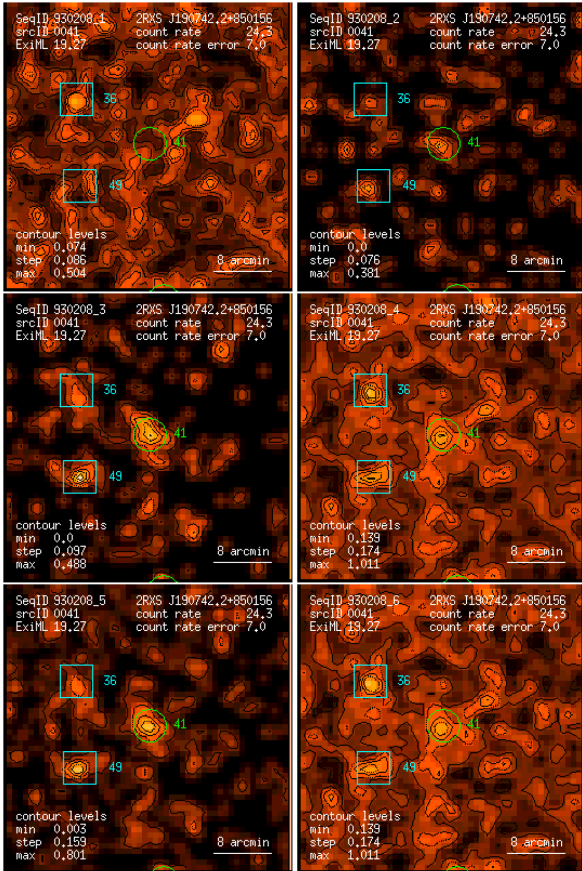
Figure 41: RASS 930208: detection 0041: band rate images, Gaussian filter: (1) PSPC channels 11 – 41, (2) 52 – 90, (3) 91 – 201, (4) 11 – 235, (5) 52 – 201, (6) 11 – 201. Broad band rates in counts/ks. Band rate contour levels in counts/ks/arcmin 2 .
