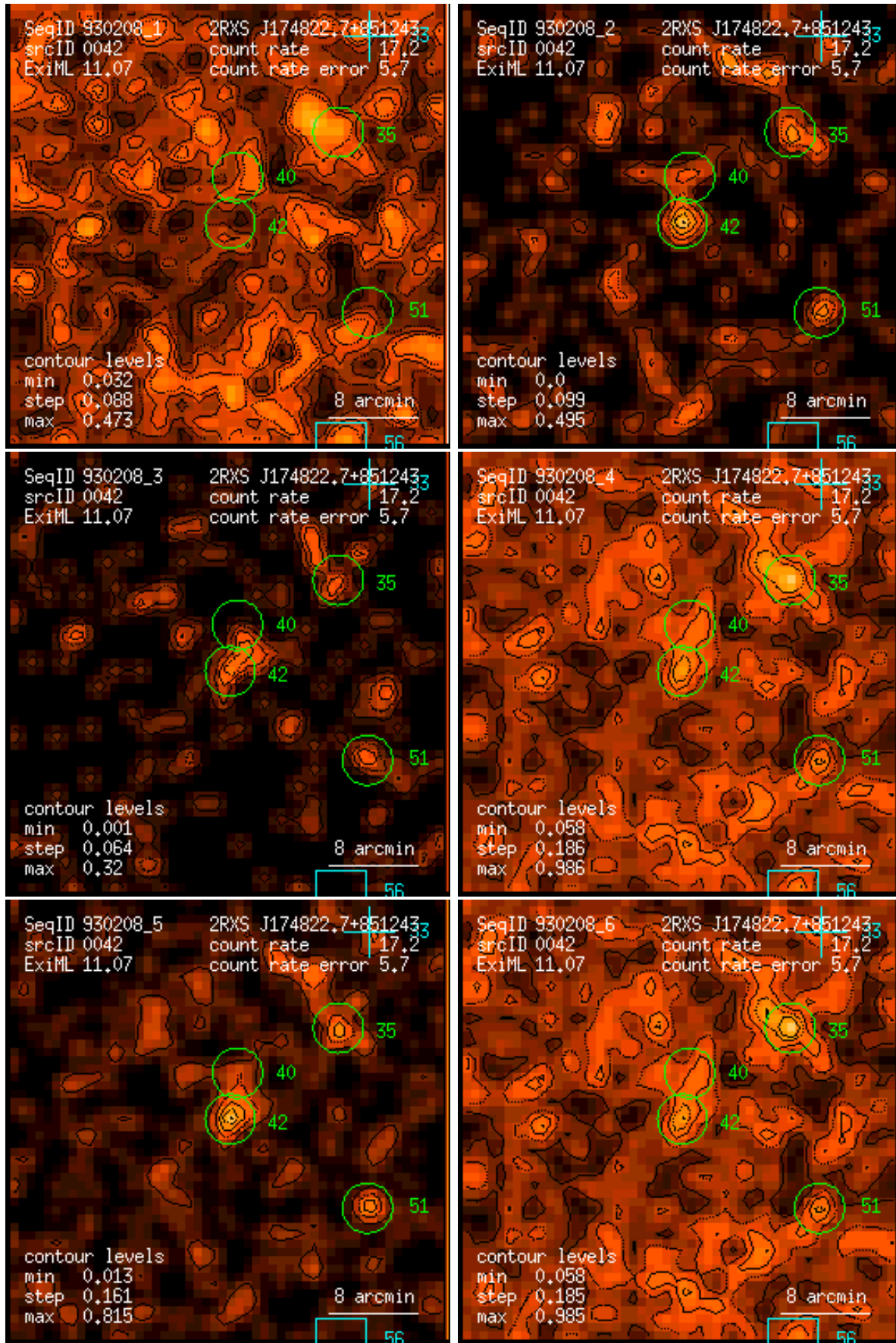
Figure 42: RASS 930208: detection 0042: band rate images, Gaussian filter: (1) PSPC channels 11 – 41, (2) 52 – 90, (3) 91 – 201, (4) 11 – 235, (5) 52 – 201, (6) 11 – 201. Broad band rates in counts/ks. Band rate contour levels in counts/ks/arcmin 2 .
