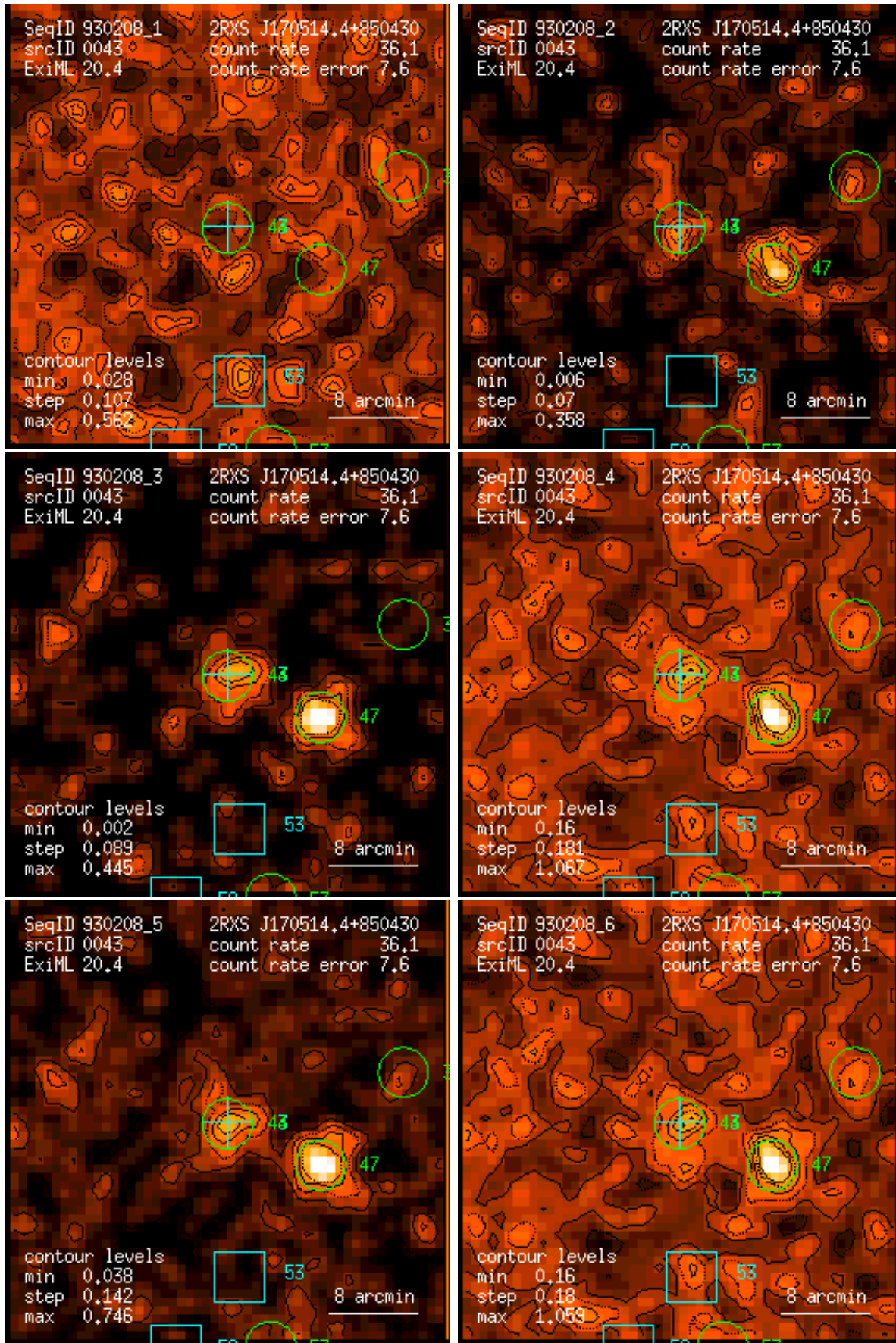
Figure 43: RASS 930208: detection 0043: band rate images, Gaussian filter: (1) PSPC channels 11 – 41, (2) 52 – 90, (3) 91 – 201, (4) 11 – 235, (5) 52 – 201, (6) 11 – 201. Broad band rates in counts/ks. Band rate contour levels in counts/ks/arcmin 2 .
