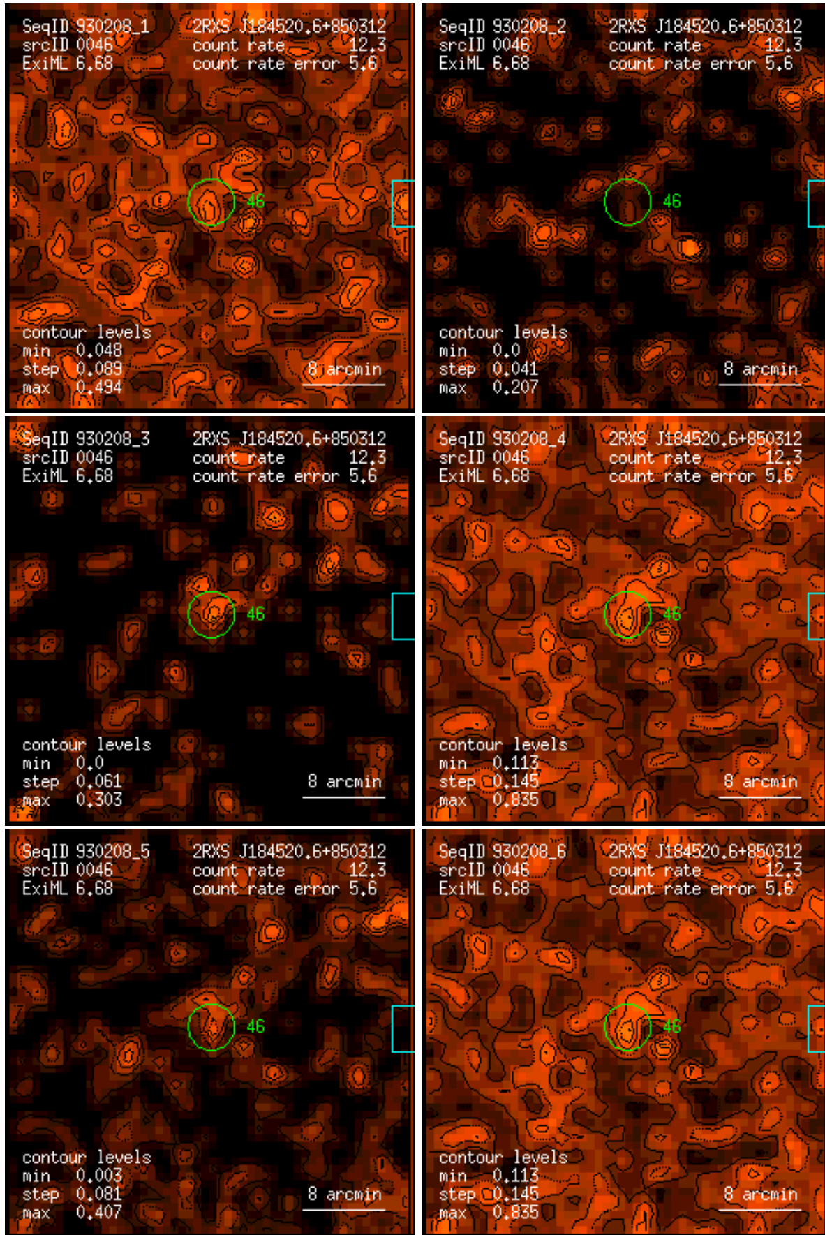
Figure 46: RASS 930208: detection 0046: band rate images, Gaussian filter: (1) PSPC channels 11 – 41, (2) 52 – 90, (3) 91 – 201, (4) 11 – 235, (5) 52 – 201, (6) 11 – 201. Broad band rates in counts/ks. Band rate contour levels in counts/ks/arcmin 2 .
