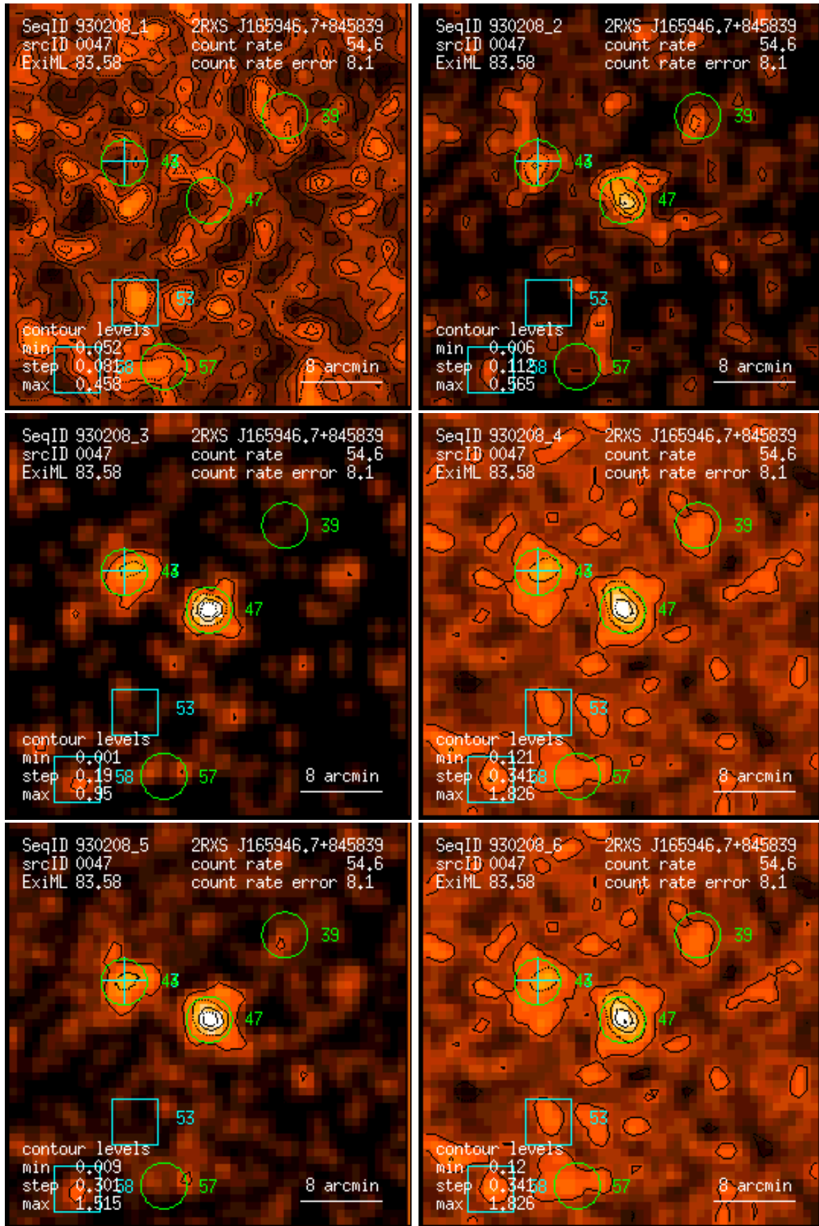
Figure 47: RASS 930208: detection 0047: band rate images, Gaussian filter: (1) PSPC channels 11 – 41, (2) 52 – 90, (3) 91 – 201, (4) 11 – 235, (5) 52 – 201, (6) 11 – 201. Broad band rates in counts/ks. Band rate contour levels in counts/ks/arcmin 2 .
