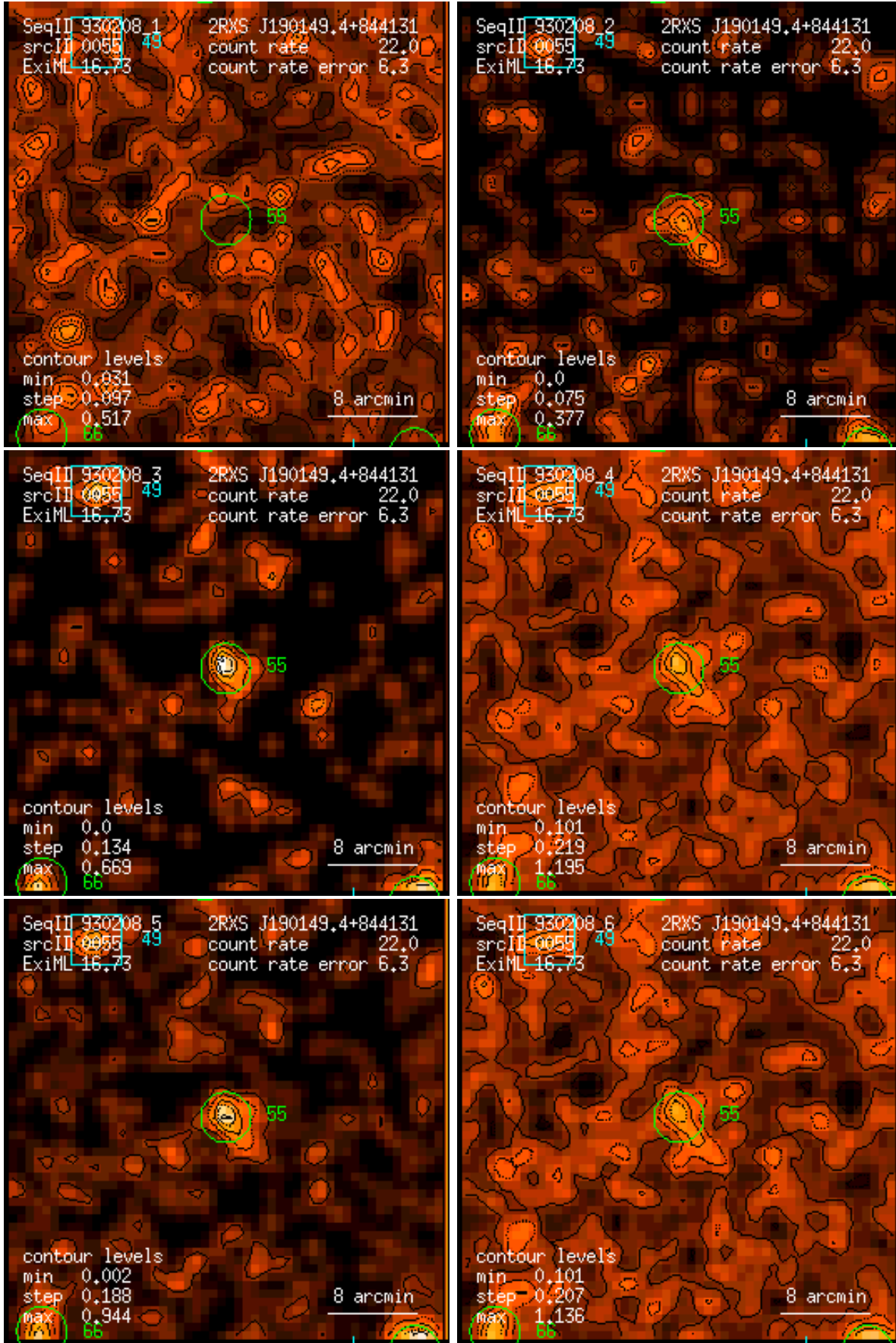
Figure 55: RASS 930208: detection 0055: band rate images, Gaussian filter: (1) PSPC channels 11 – 41, (2) 52 – 90, (3) 91 – 201, (4) 11 – 235, (5) 52 – 201, (6) 11 – 201. Broad band rates in counts/ks. Band rate contour levels in counts/ks/arcmin 2 .
