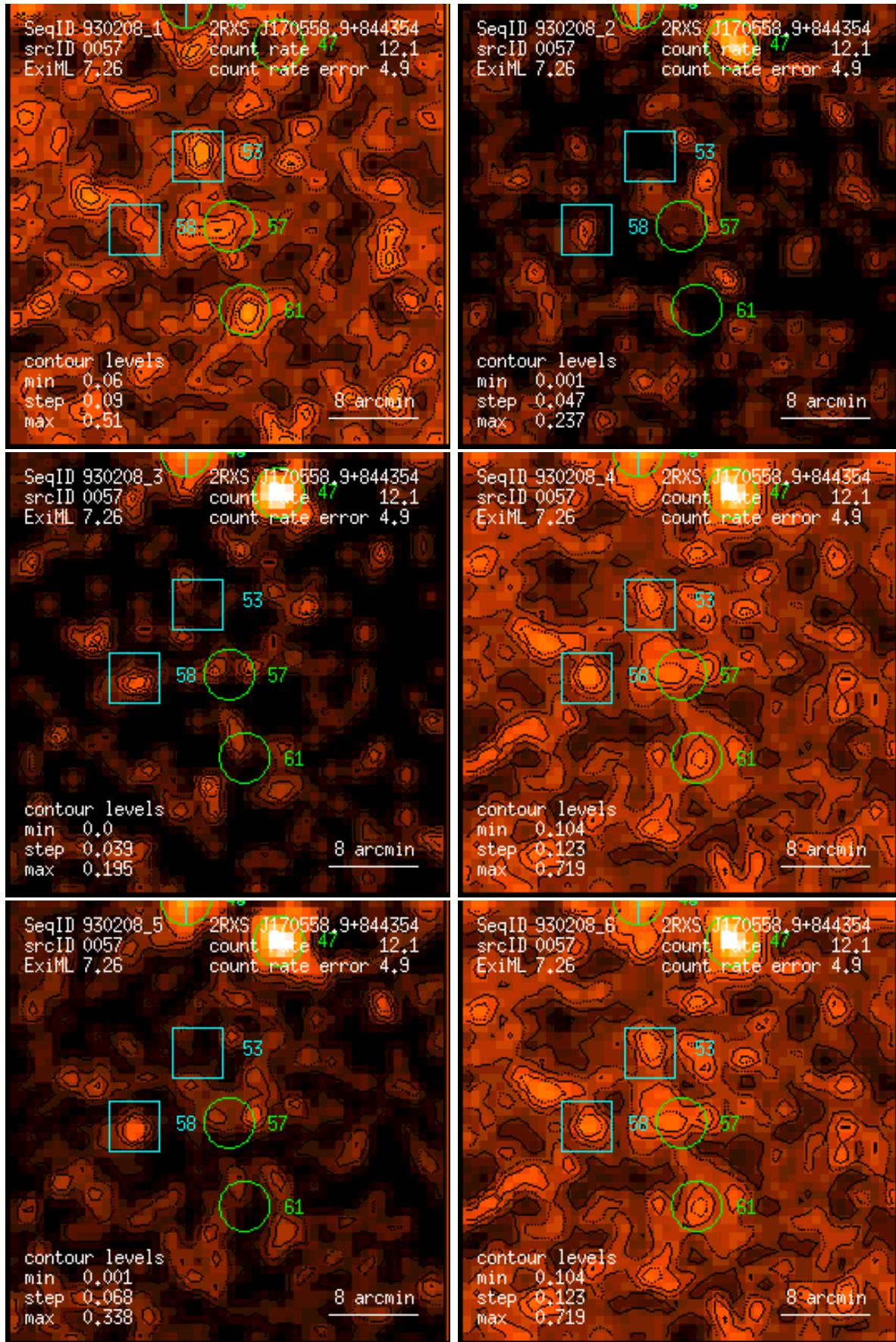
Figure 57: RASS 930208: detection 0057: band rate images, Gaussian filter: (1) PSPC channels 11 – 41, (2) 52 – 90, (3) 91 – 201, (4) 11 – 235, (5) 52 – 201, (6) 11 – 201. Broad band rates in counts/ks. Band rate contour levels in counts/ks/arcmin 2 .
