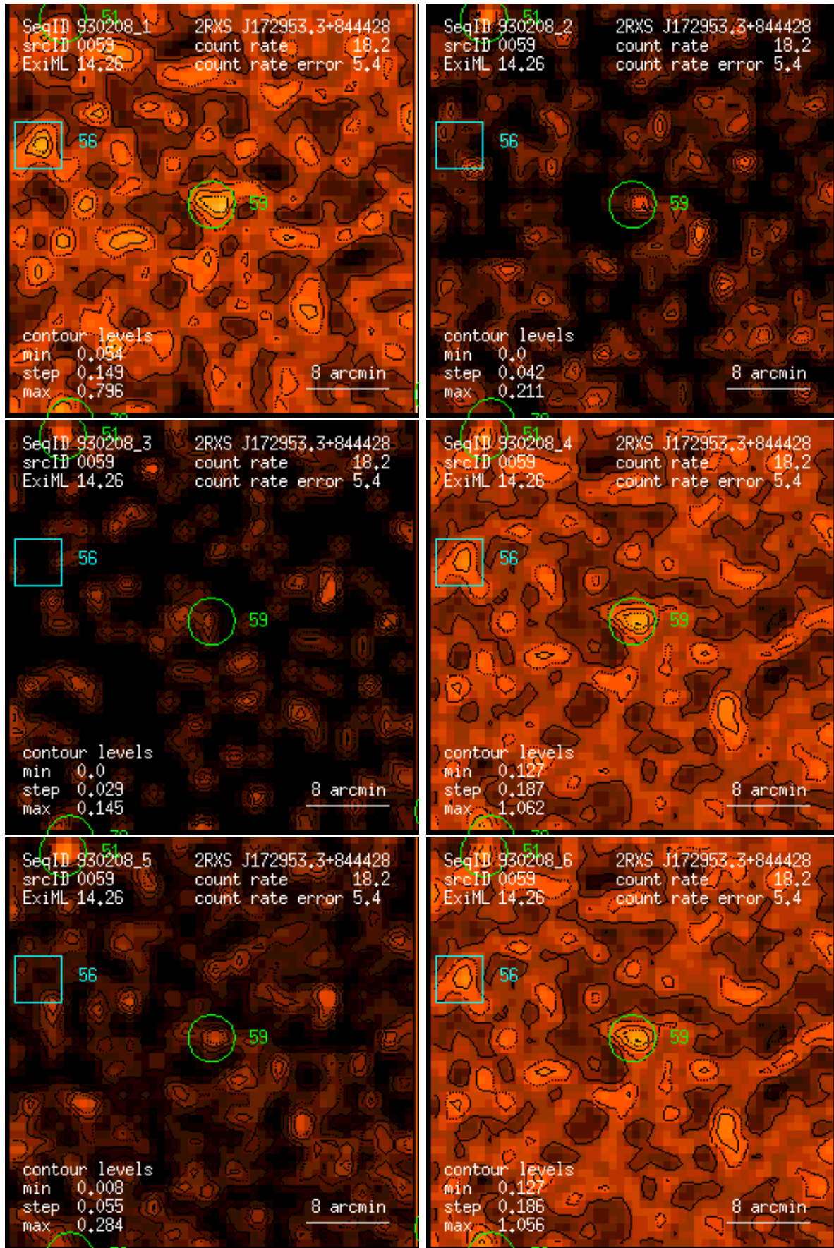
Figure 59: RASS 930208: detection 0059: band rate images, Gaussian filter: (1) PSPC channels 11 – 41, (2) 52 – 90, (3) 91 – 201, (4) 11 – 235, (5) 52 – 201, (6) 11 – 201. Broad band rates in counts/ks. Band rate contour levels in counts/ks/arcmin 2 .
