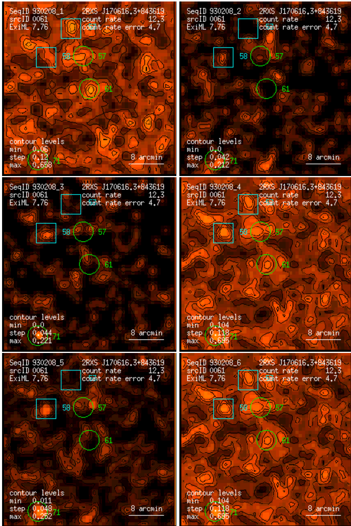
Figure 61: RASS 930208: detection 0061: band rate images, Gaussian filter: (1) PSPC channels 11 – 41, (2) 52 – 90, (3) 91 – 201, (4) 11 – 235, (5) 52 – 201, (6) 11 – 201. Broad band rates in counts/ks. Band rate contour levels in counts/ks/arcmin 2 .
