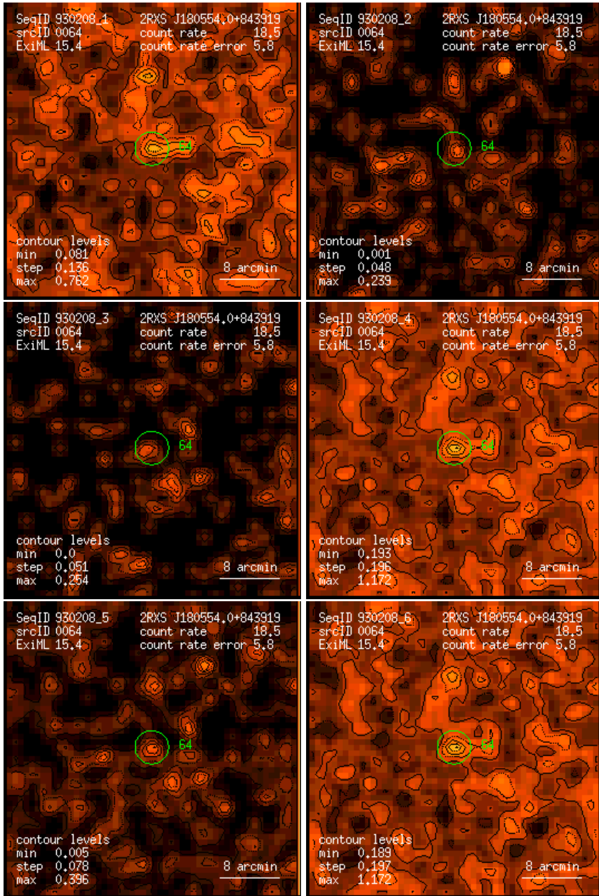
Figure 64: RASS 930208: detection 0064: band rate images, Gaussian filter: (1) PSPC channels 11 – 41, (2) 52 – 90, (3) 91 – 201, (4) 11 – 235, (5) 52 – 201, (6) 11 – 201. Broad band rates in counts/ks. Band rate contour levels in counts/ks/arcmin 2 .
