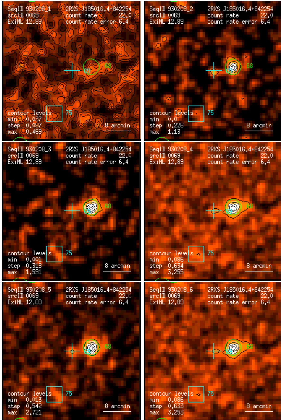
Figure 69: RASS 930208: detection 0069: band rate images, Gaussian filter: (1) PSPC channels 11 – 41, (2) 52 – 90, (3) 91 – 201, (4) 11 – 235, (5) 52 – 201, (6) 11 – 201. Broad band rates in counts/ks. Band rate contour levels in counts/ks/arcmin 2 .
