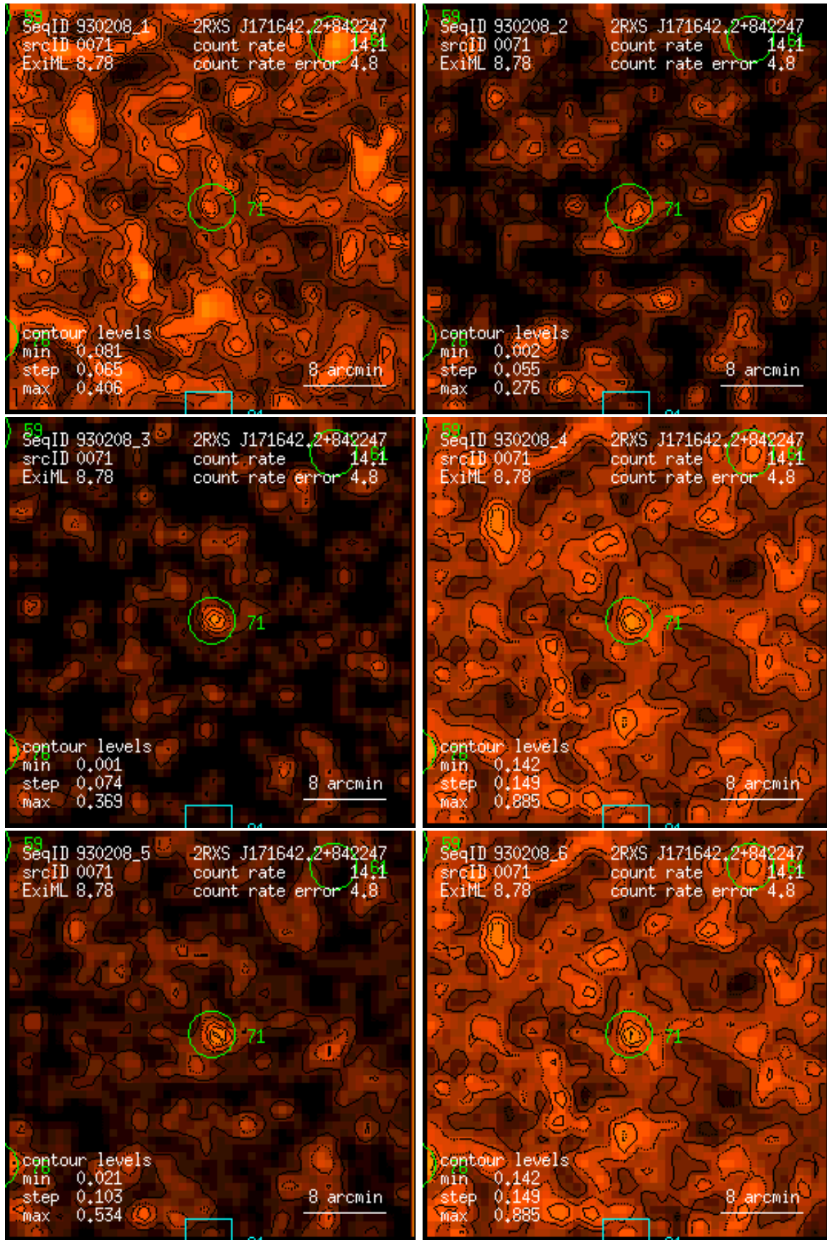
Figure 71: RASS 930208: detection 0071: band rate images, Gaussian filter: (1) PSPC channels 11 – 41, (2) 52 – 90, (3) 91 – 201, (4) 11 – 235, (5) 52 – 201, (6) 11 – 201. Broad band rates in counts/ks. Band rate contour levels in counts/ks/arcmin 2 .
