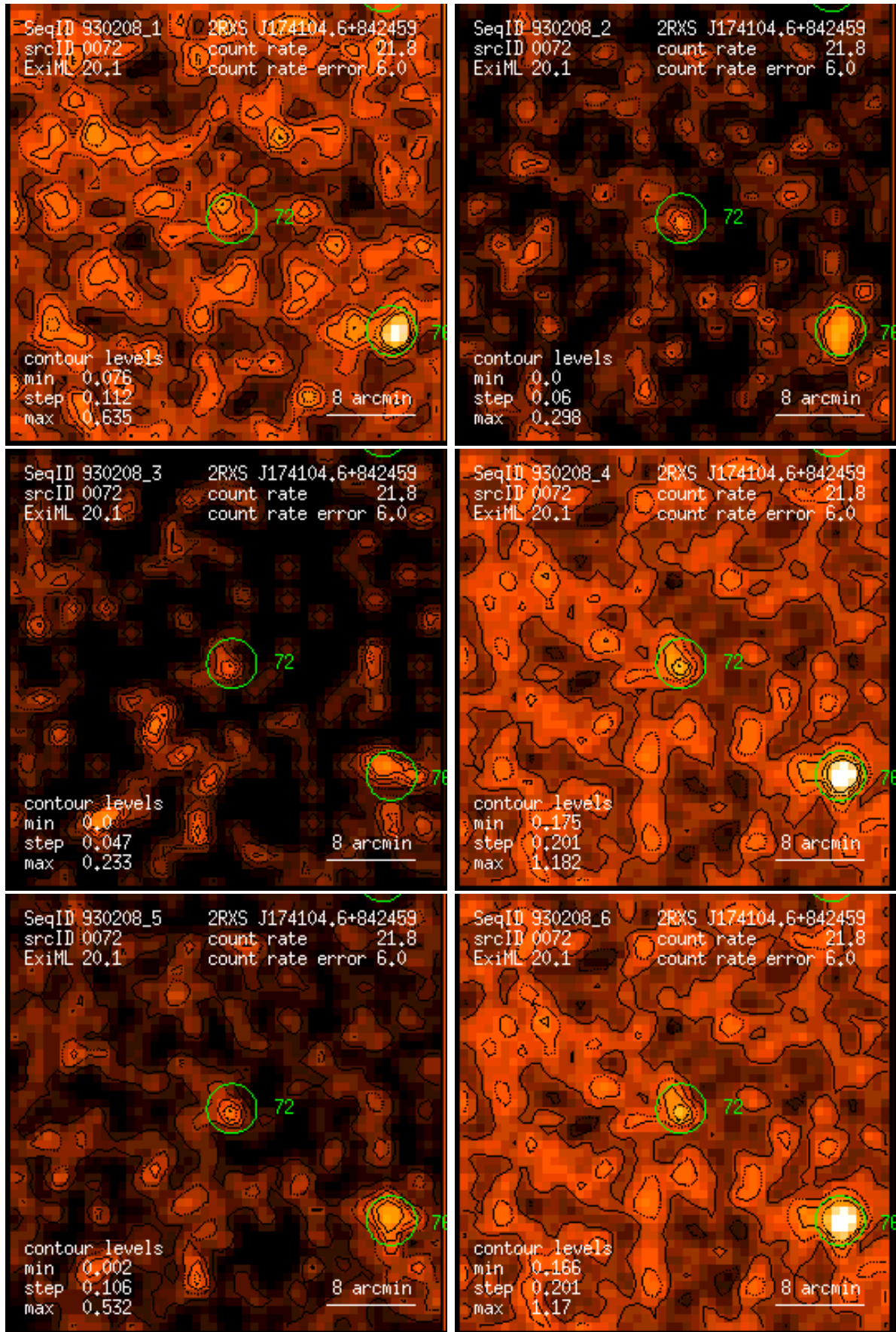
Figure 72: RASS 930208: detection 0072: band rate images, Gaussian filter: (1) PSPC channels 11 – 41, (2) 52 – 90, (3) 91 – 201, (4) 11 – 235, (5) 52 – 201, (6) 11 – 201. Broad band rates in counts/ks. Band rate contour levels in counts/ks/arcmin 2 .
