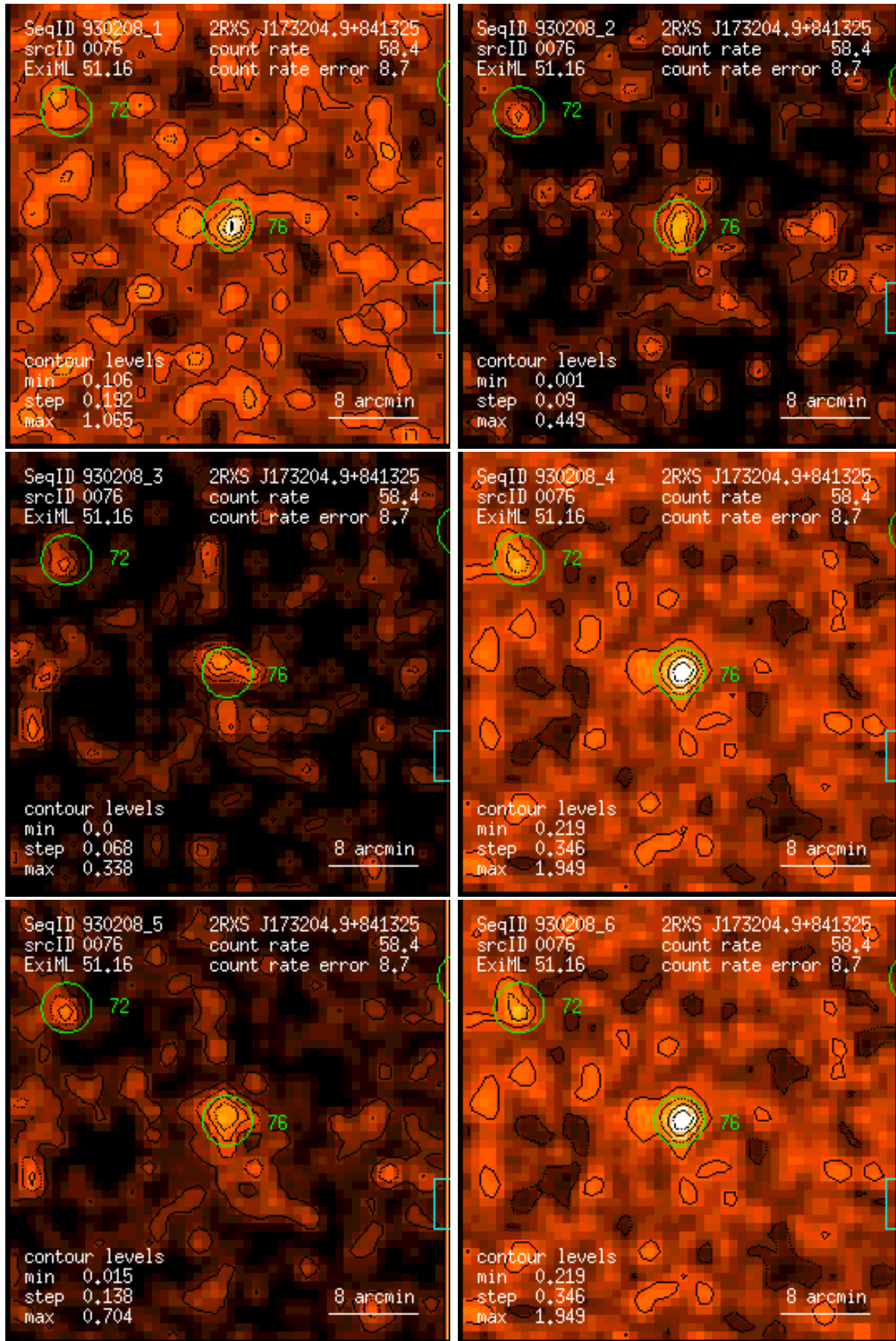
Figure 76: RASS 930208: detection 0076: band rate images, Gaussian filter: (1) PSPC channels 11 – 41, (2) 52 – 90, (3) 91 – 201, (4) 11 – 235, (5) 52 – 201, (6) 11 – 201. Broad band rates in counts/ks. Band rate contour levels in counts/ks/arcmin 2 .
