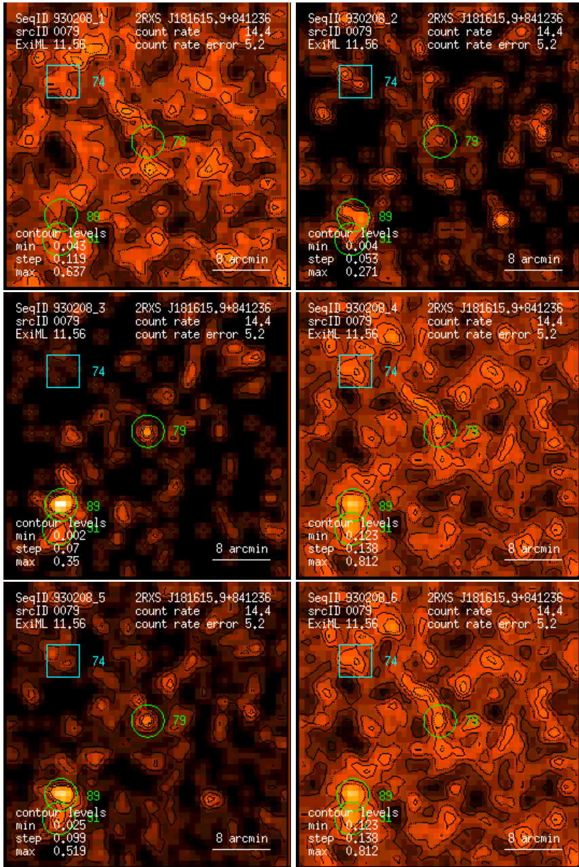
Figure 79: RASS 930208: detection 0079: band rate images, Gaussian filter: (1) PSPC channels 11 – 41, (2) 52 – 90, (3) 91 – 201, (4) 11 – 235, (5) 52 – 201, (6) 11 – 201. Broad band rates in counts/ks. Band rate contour levels in counts/ks/arcmin 2 .
