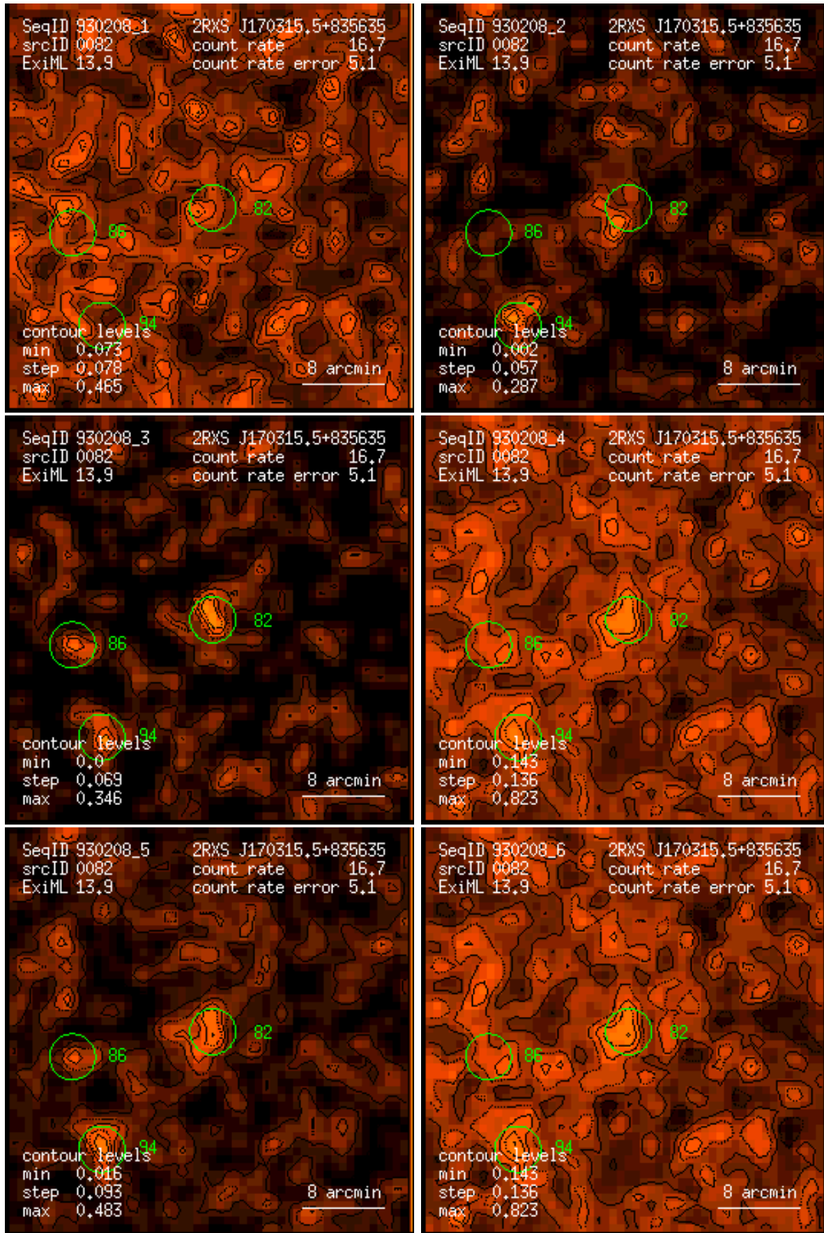
Figure 82: RASS 930208: detection 0082: band rate images, Gaussian filter: (1) PSPC channels 11 – 41, (2) 52 – 90, (3) 91 – 201, (4) 11 – 235, (5) 52 – 201, (6) 11 – 201. Broad band rates in counts/ks. Band rate contour levels in counts/ks/arcmin 2 .
