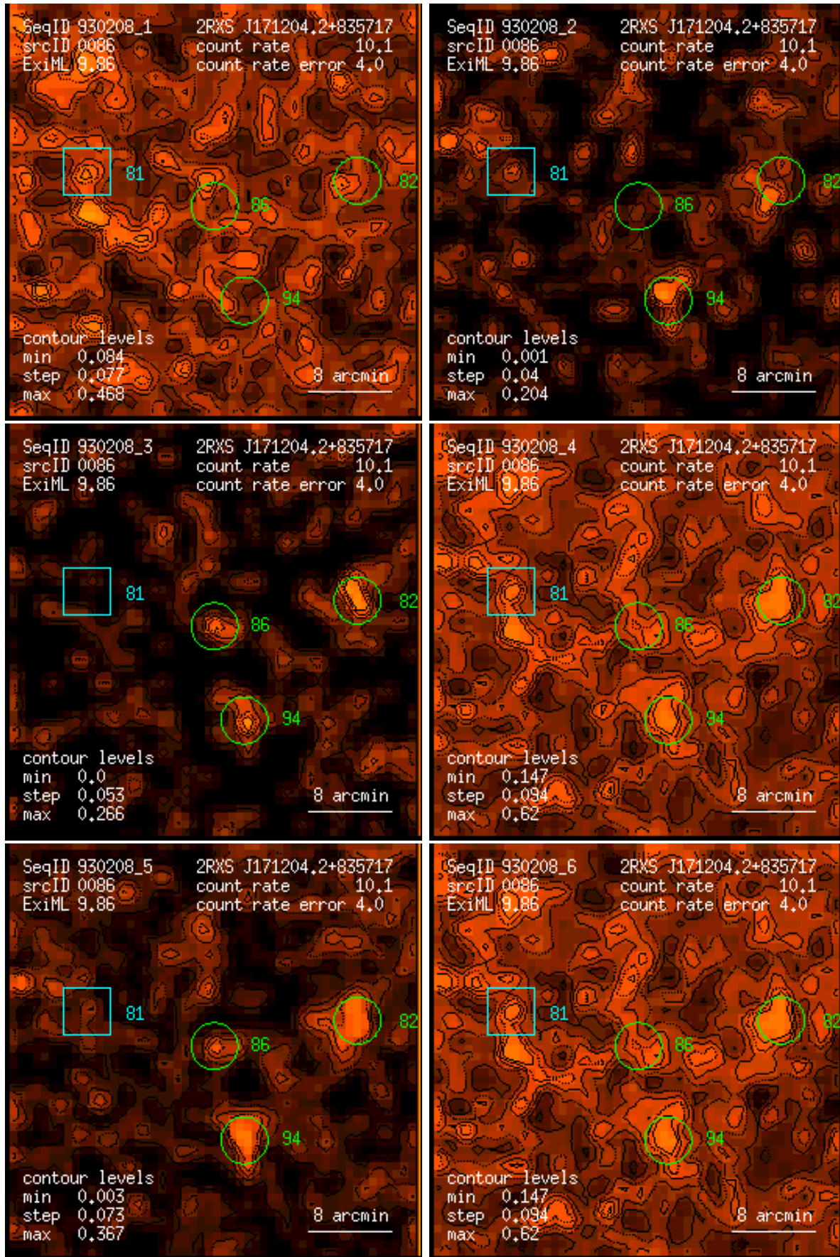
Figure 86: RASS 930208: detection 0086: band rate images, Gaussian filter: (1) PSPC channels 11 – 41, (2) 52 – 90, (3) 91 – 201, (4) 11 – 235, (5) 52 – 201, (6) 11 – 201. Broad band rates in counts/ks. Band rate contour levels in counts/ks/arcmin 2 .
