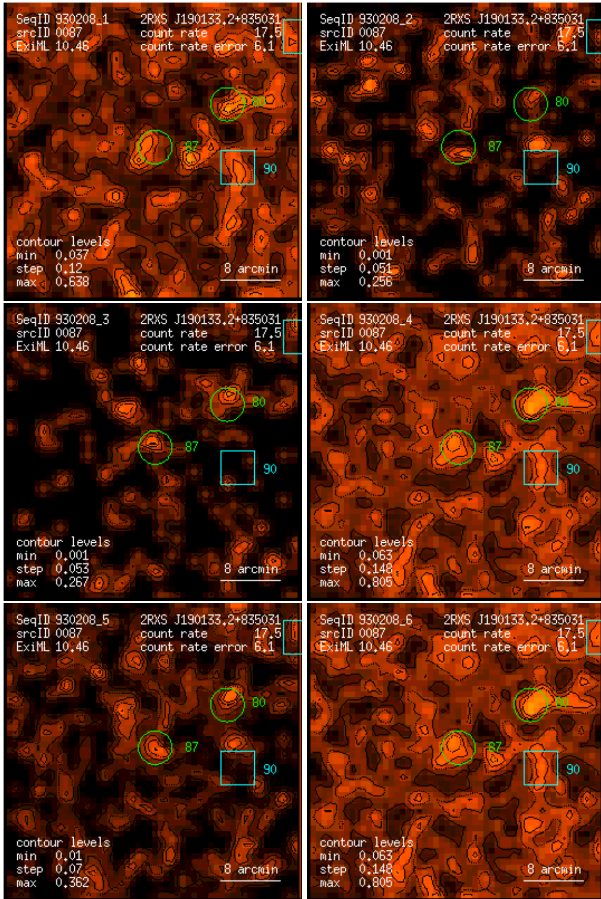
Figure 87: RASS 930208: detection 0087: band rate images, Gaussian filter: (1) PSPC channels 11 – 41, (2) 52 – 90, (3) 91 – 201, (4) 11 – 235, (5) 52 – 201, (6) 11 – 201. Broad band rates in counts/ks. Band rate contour levels in counts/ks/arcmin 2 .
