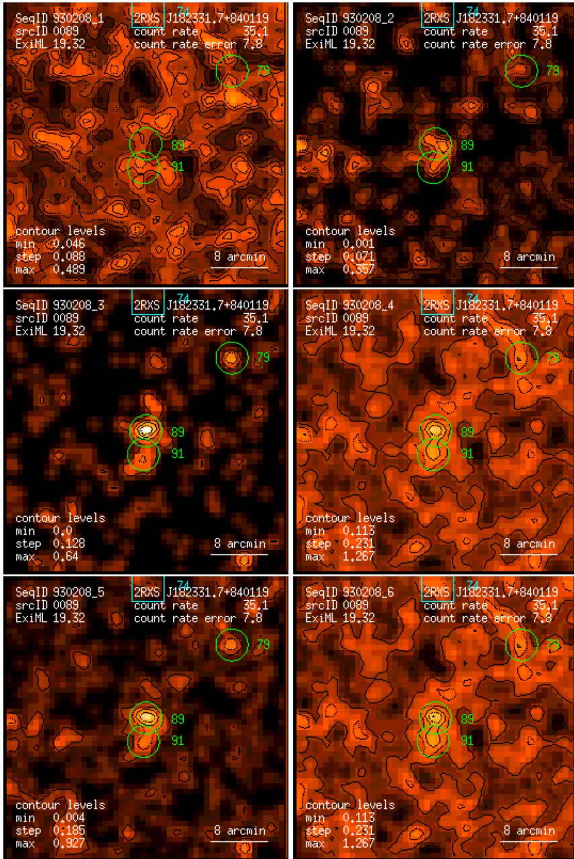
Figure 89: RASS 930208: detection 0089: band rate images, Gaussian filter: (1) PSPC channels 11 – 41, (2) 52 – 90, (3) 91 – 201, (4) 11 – 235, (5) 52 – 201, (6) 11 – 201. Broad band rates in counts/ks. Band rate contour levels in counts/ks/arcmin 2 .
