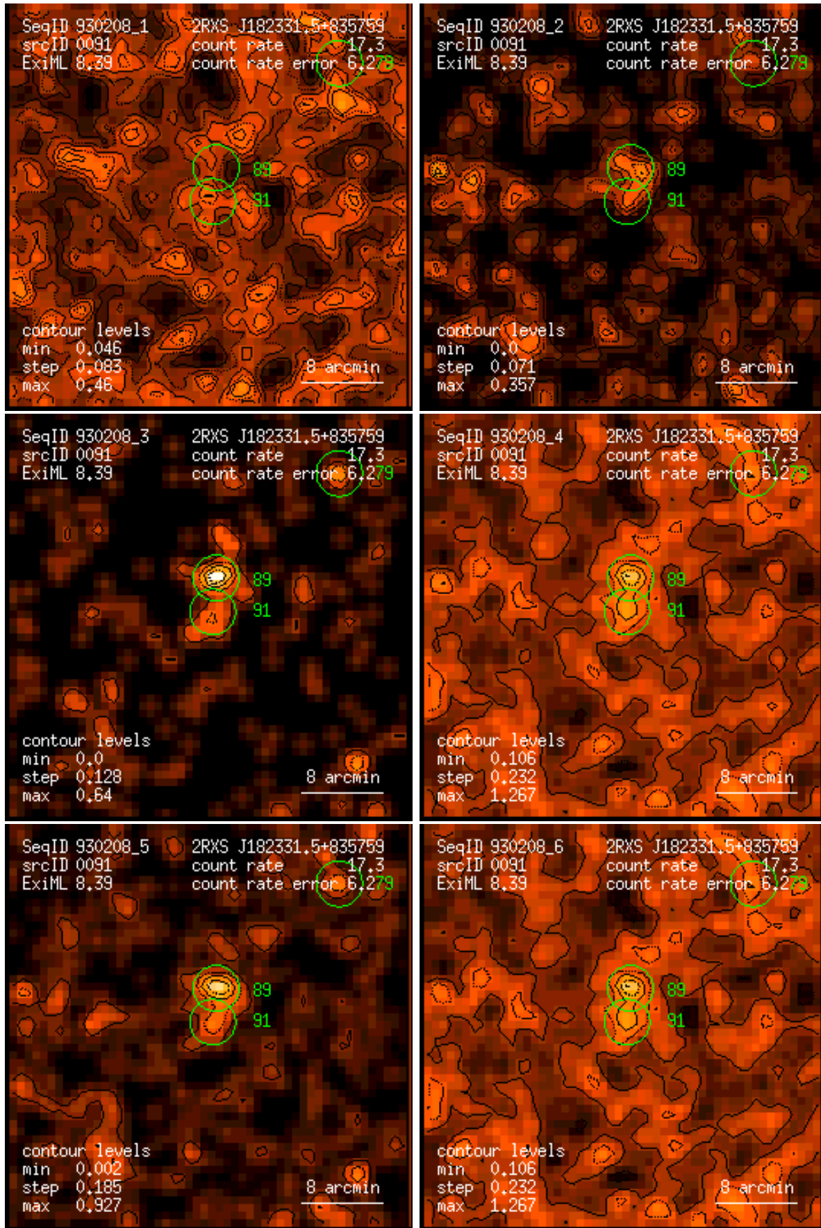
Figure 91: RASS 930208: detection 0091: band rate images, Gaussian filter: (1) PSPC channels 11 – 41, (2) 52 – 90, (3) 91 – 201, (4) 11 – 235, (5) 52 – 201, (6) 11 – 201. Broad band rates in counts/ks. Band rate contour levels in counts/ks/arcmin 2 .
