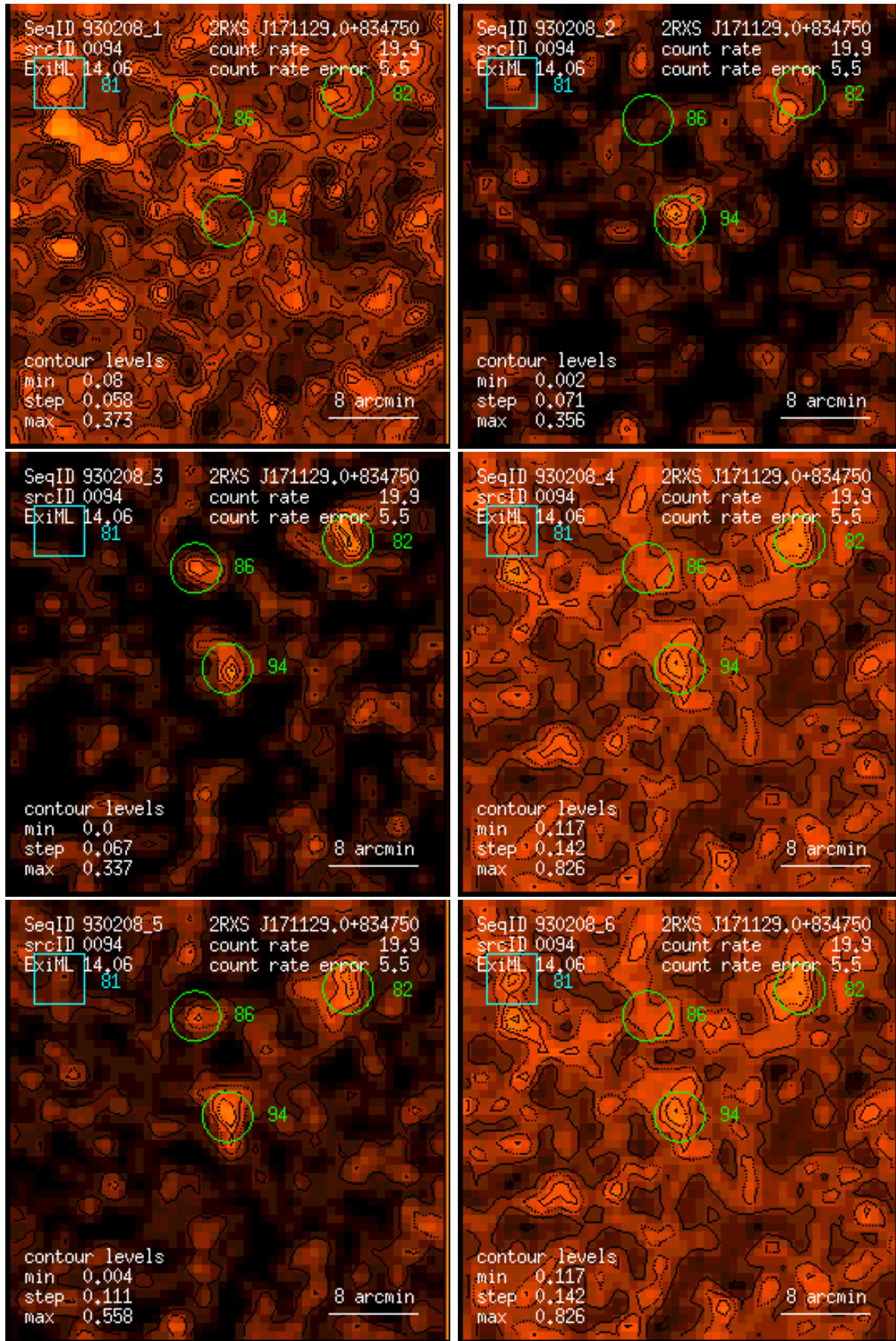
Figure 94: RASS 930208: detection 0094: band rate images, Gaussian filter: (1) PSPC channels 11 – 41, (2) 52 – 90, (3) 91 – 201, (4) 11 – 235, (5) 52 – 201, (6) 11 – 201. Broad band rates in counts/ks. Band rate contour levels in counts/ks/arcmin 2 .
