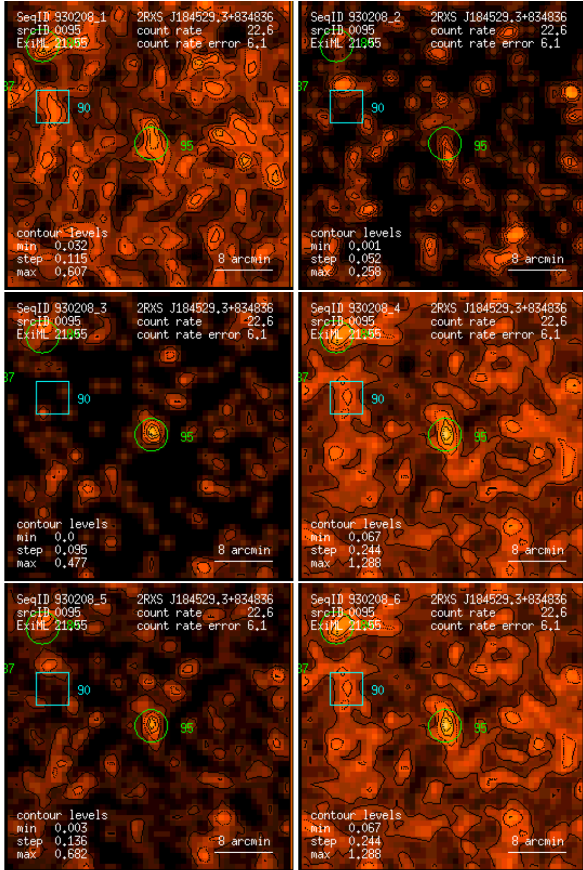
Figure 95: RASS 930208: detection 0095: band rate images, Gaussian filter: (1) PSPC channels 11 – 41, (2) 52 – 90, (3) 91 – 201, (4) 11 – 235, (5) 52 – 201, (6) 11 – 201. Broad band rates in counts/ks. Band rate contour levels in counts/ks/arcmin 2 .
