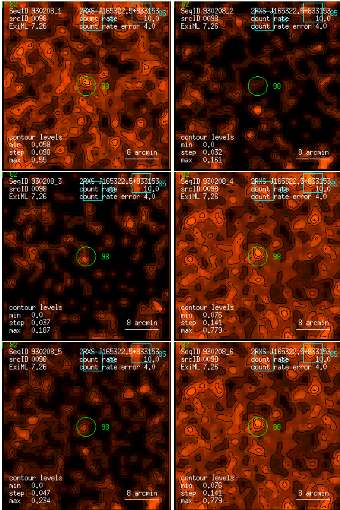
Figure 98: RASS 930208: detection 0098: band rate images, Gaussian filter: (1) PSPC channels 11 – 41, (2) 52 – 90, (3) 91 – 201, (4) 11 – 235, (5) 52 – 201, (6) 11 – 201. Broad band rates in counts/ks. Band rate contour levels in counts/ks/arcmin 2 .
