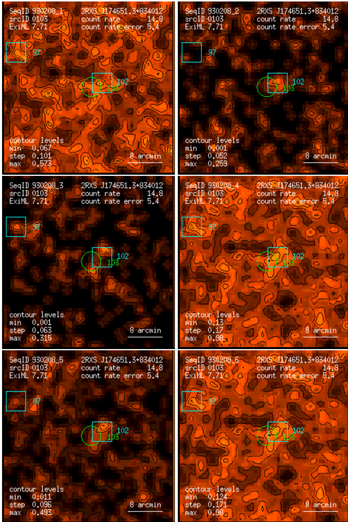
Figure 103: RASS 930208: detection 0103: band rate images, Gaussian filter: (1) PSPC channels 11 – 41, (2) 52 – 90, (3) 91 – 201, (4) 11 – 235, (5) 52 – 201, (6) 11 – 201. Broad band rates in counts/ks. Band rate contour levels in counts/ks/arcmin 2 .
