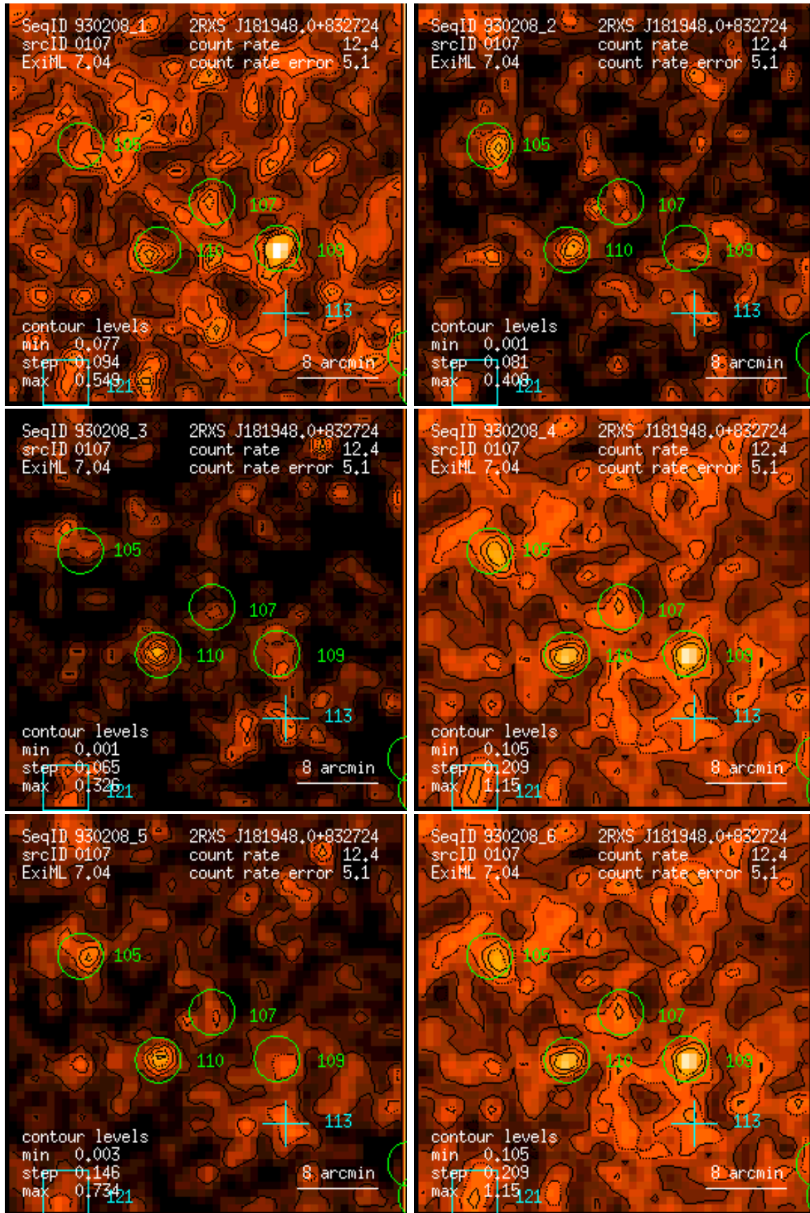
Figure 107: RASS 930208: detection 0107: band rate images, Gaussian filter: (1) PSPC channels 11 – 41, (2) 52 – 90, (3) 91 – 201, (4) 11 – 235, (5) 52 – 201, (6) 11 – 201. Broad band rates in counts/ks. Band rate contour levels in counts/ks/arcmin 2 .
